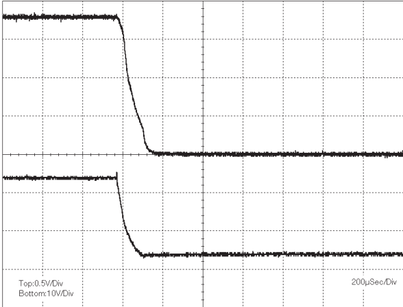
Figure 10: Turn-Off Characteristic
