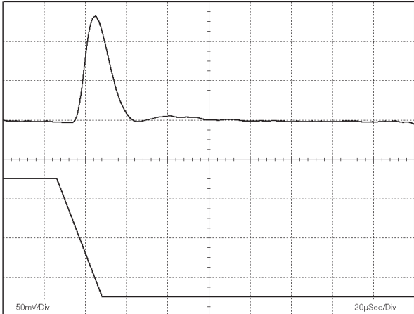
Figure 16: Typical Transient Response 75-50% Step Load Change (1 A/ s), Top (Vout) Bottom (Iout)
