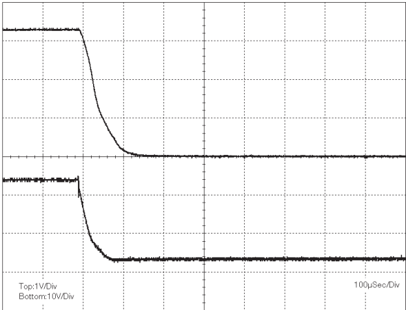
Figure 20: Turn-Off Characteristic
