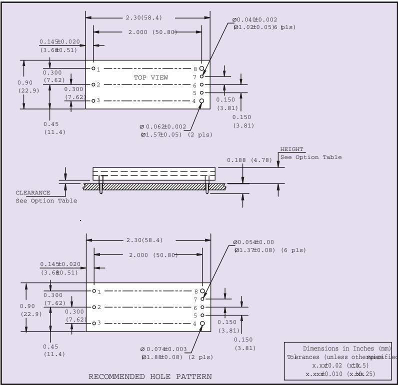
Figure 21 - Through-hole Mechanical Drawing, Dimension Options and Pinout Table
