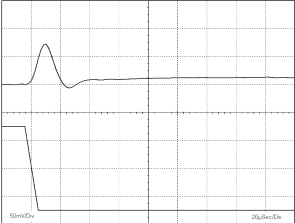
Figure 6: Typical Transient Response 75-50% Step Load Change (1 A/ \mu s), Top (Vout) Bottom (Iout)
