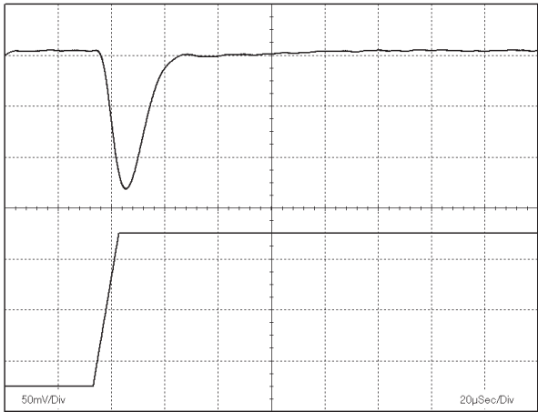
Figure 17: Typical Transient Response 50-75% Step Load Change (1 A/ s), Top (Vout) Bottom (Iout)
