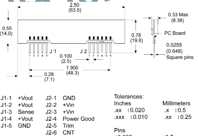
APA06 ( Buck ) Pinout
