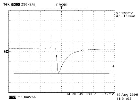
Figure 8: Output deviation from 50% to 75% load change, V_{IN} = 48 \text{ Vdc} , T_A = 25^\circ\text{C} .
