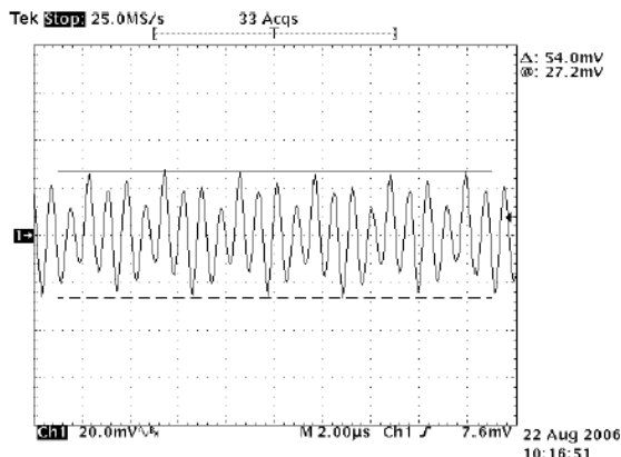
Figure 7: Output ripple and noise, V_{IN} = 48 \text{ Vdc} , I_O = 20 \text{ A} , T_A = 85^\circ\text{C} .
