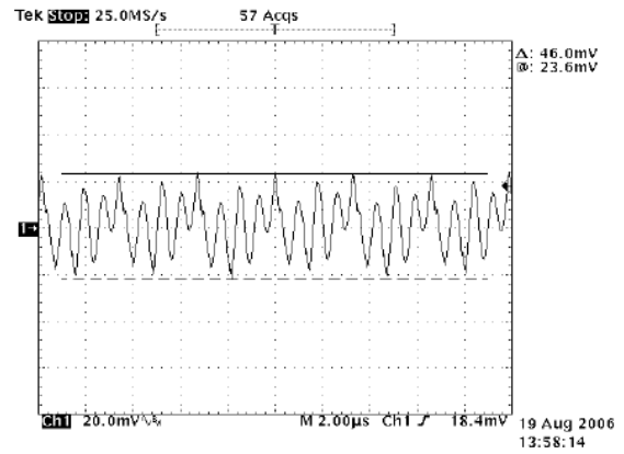
Figure 6: Output ripple and noise, V_{IN} = 48 \text{ Vdc} , I_O = 20 \text{ A} , T_A = 25^\circ\text{C} .
