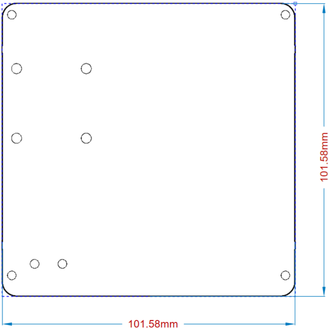
Board outline
