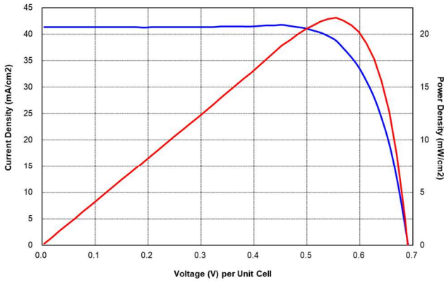
Current-Voltage Characteristics
