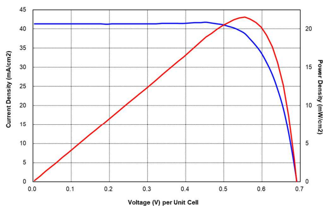
Current-Voltage Characteristics
