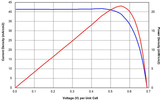
Current-Voltage Characteristics
