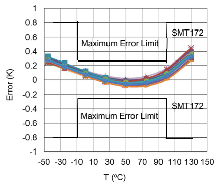
Accuracy vs. Temperature (TO18 V_{CC}=5V )
