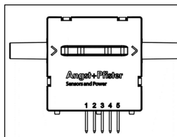
Figure 2 Digital and analog version (I 2 C) pin assignment
