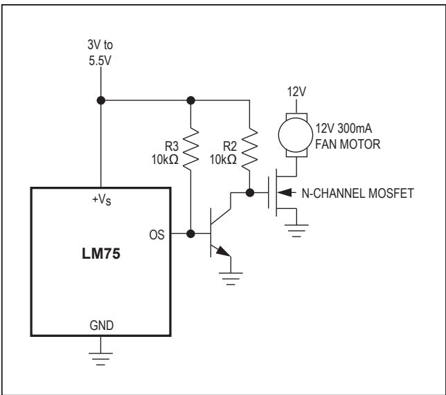
Figure 8. Fan Control
