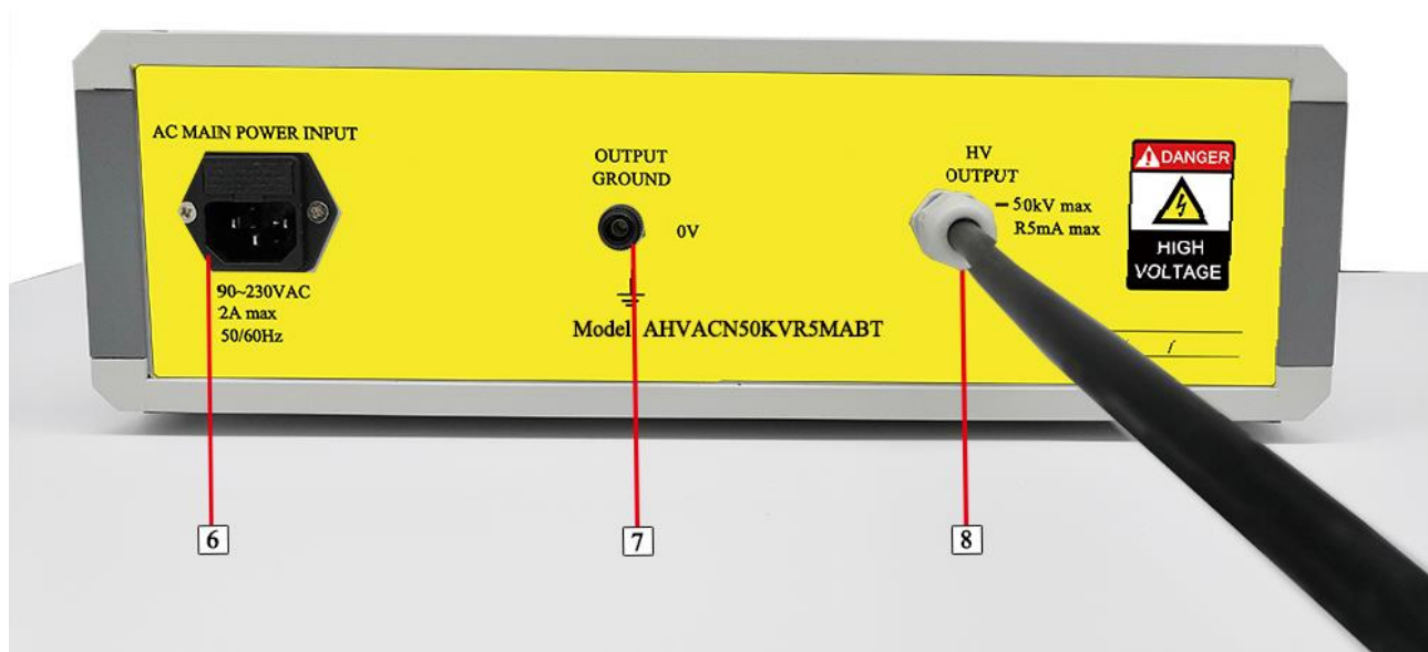
Figure 3. Back Panel
