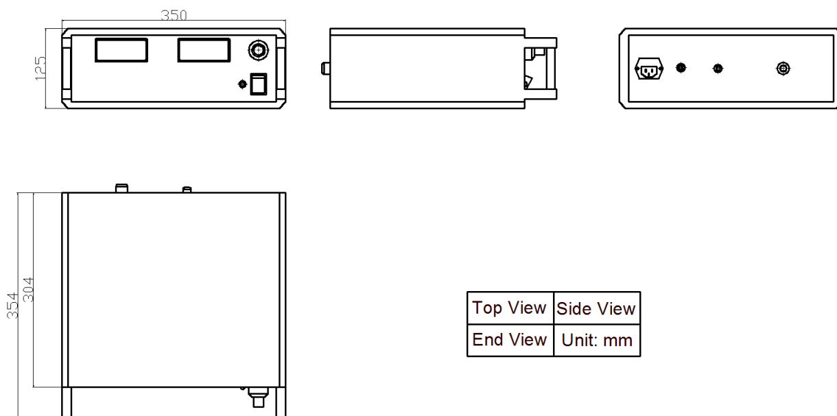
Figure 7. Dimensions for AHVACN10KV10MABT
