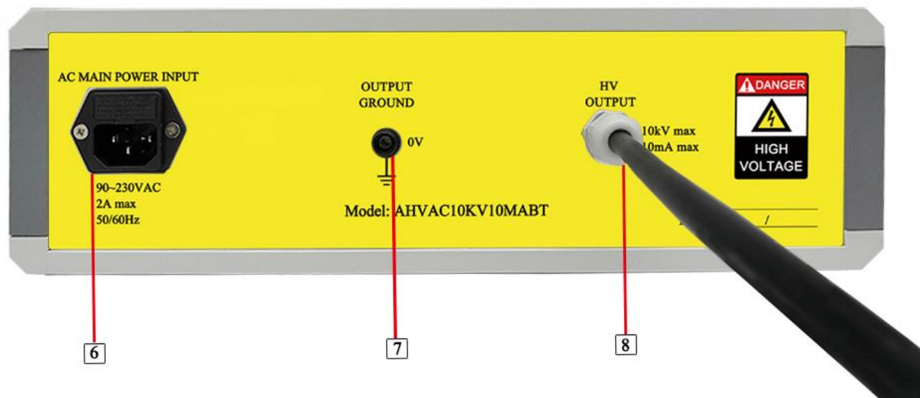
Figure 3. Back Panel
