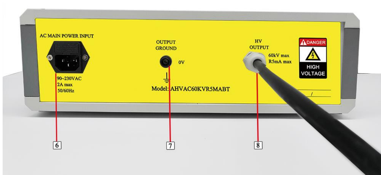
Figure 3. Back Panel
