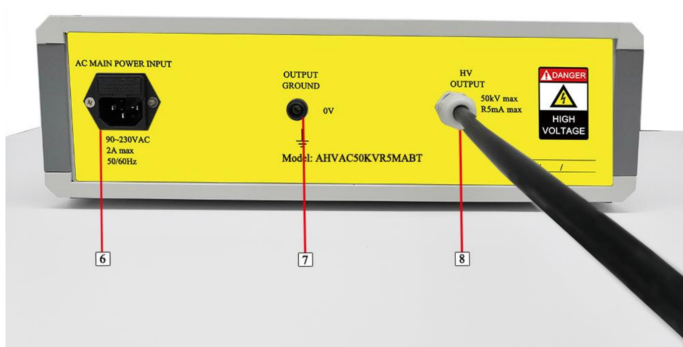
Figure 3. Back Panel
