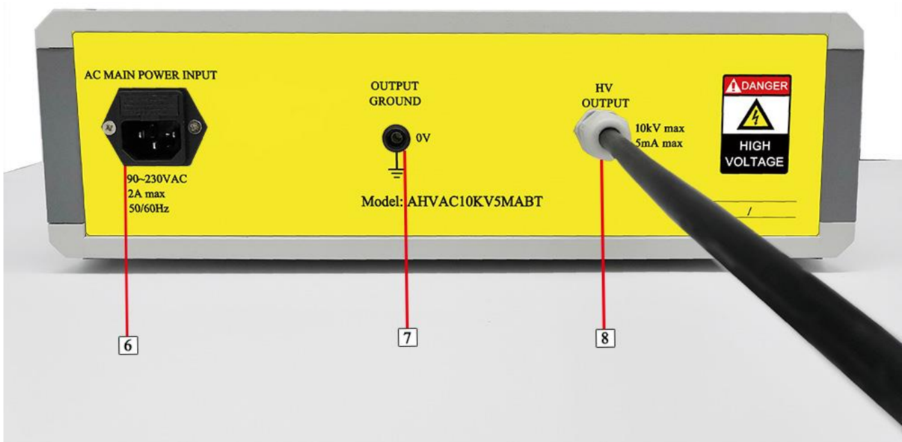
Figure 3. Back Panel
