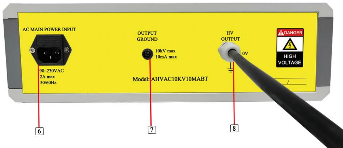
Figure 3. Back Panel
