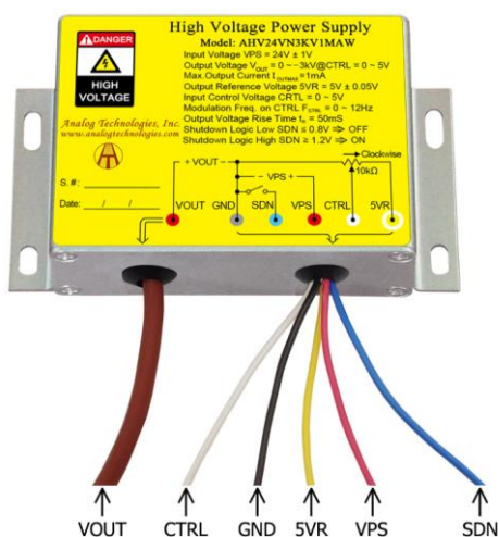
Figure 2. The Connecting Lead Wires of AHV24VN3KV1MAW
