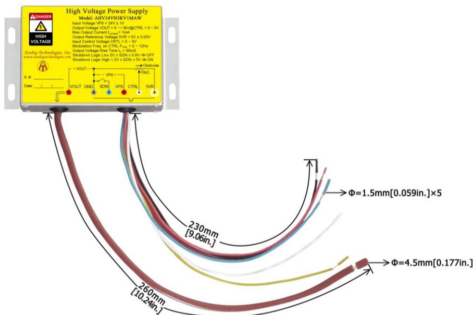
Figure 13. Connecting Lead Wires of AHV24VN3KV1MAW
