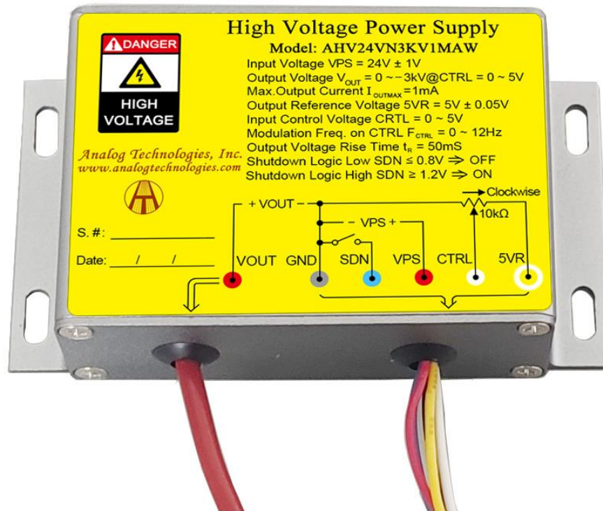
Figure 1.1. Top View of AHV24VN3KV1MAW
