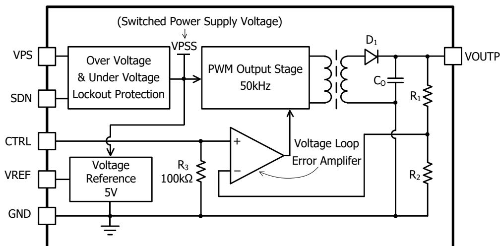
High Voltage Power Supply Function Block Diagram
