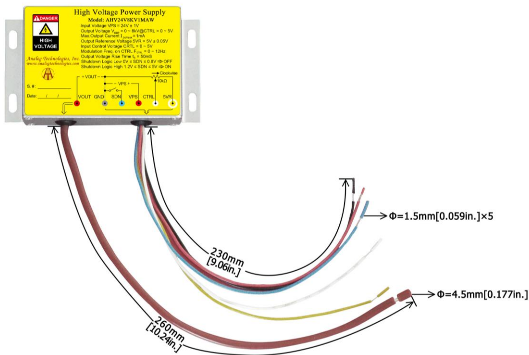
Figure 13. Connecting Lead Wires of AHV24V8KV1MAW
