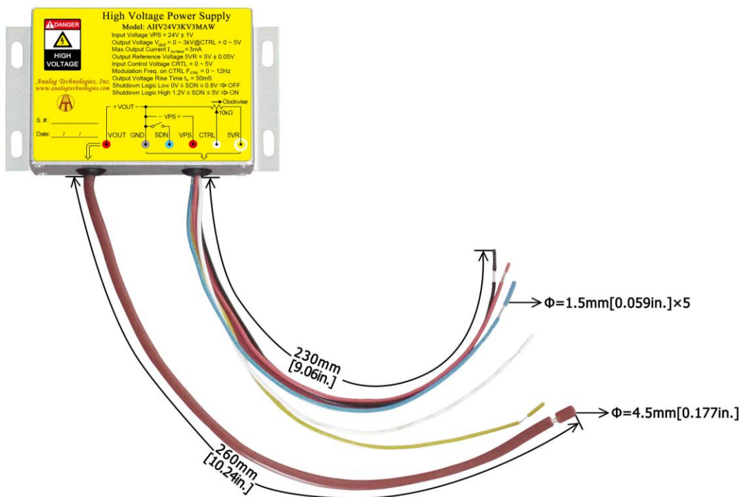
Figure 13. Connecting Lead Wires of AHV24V3KV3MAW
