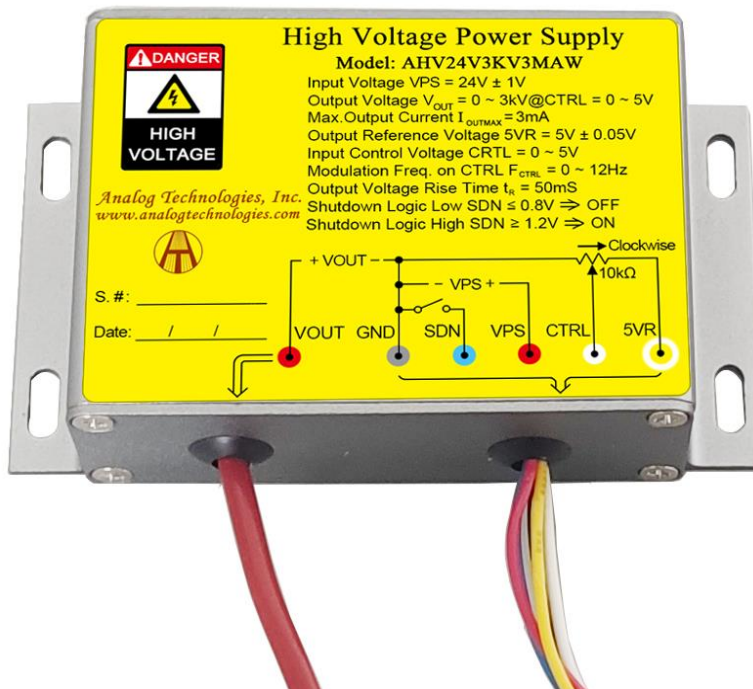
Figure 1.1. Top View of AHV24V3KV3MAW
