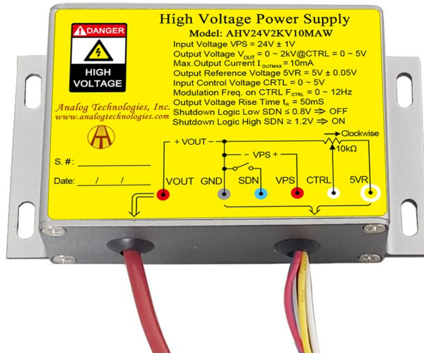
Figure 1.1. Top View of AHV24V2KV10MAW
