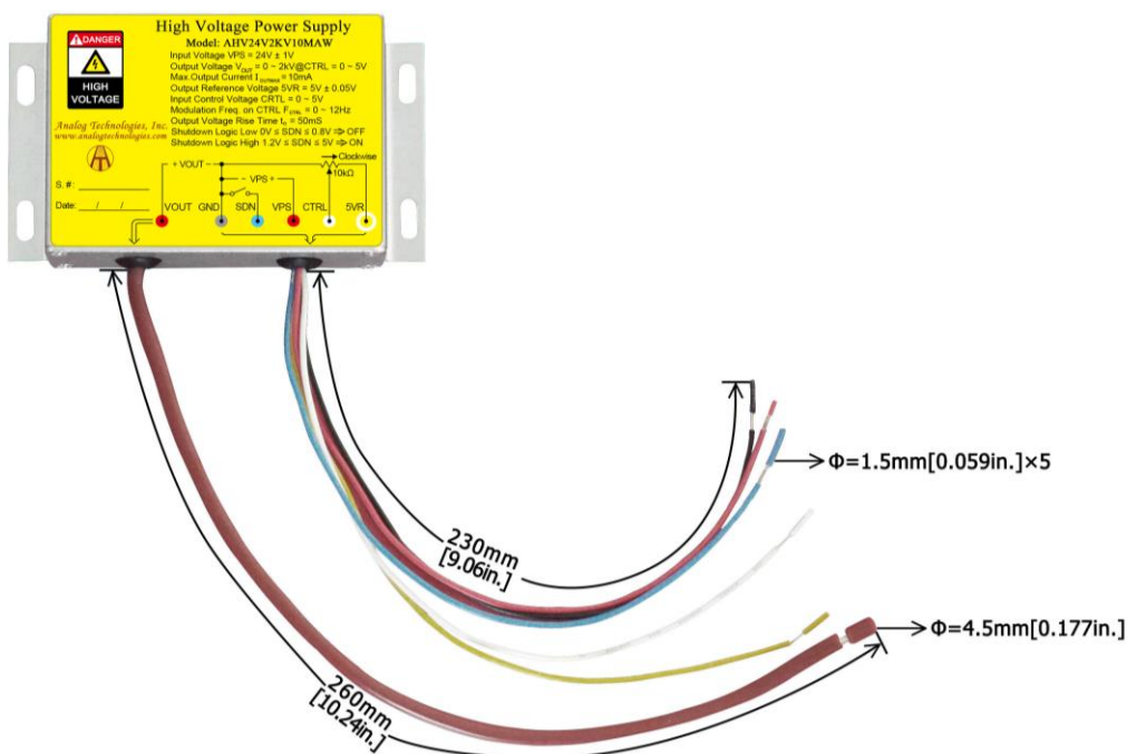
Figure 13. Connecting Lead Wires of AHV24V2KV10MAW
