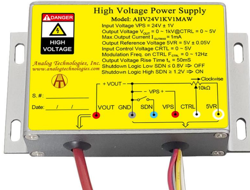
Figure 1.1. Top View of AHV24V1KV1MAW
