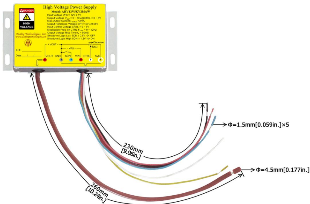
Figure 13. Connecting Lead Wires of AHV12V5KV2MAW
