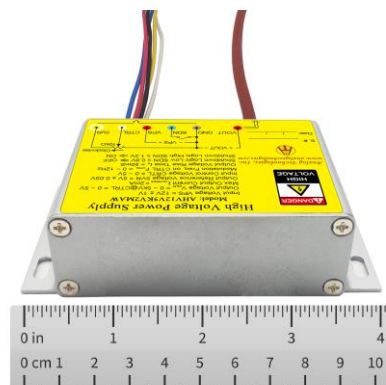
Figure 1.3. Side View
