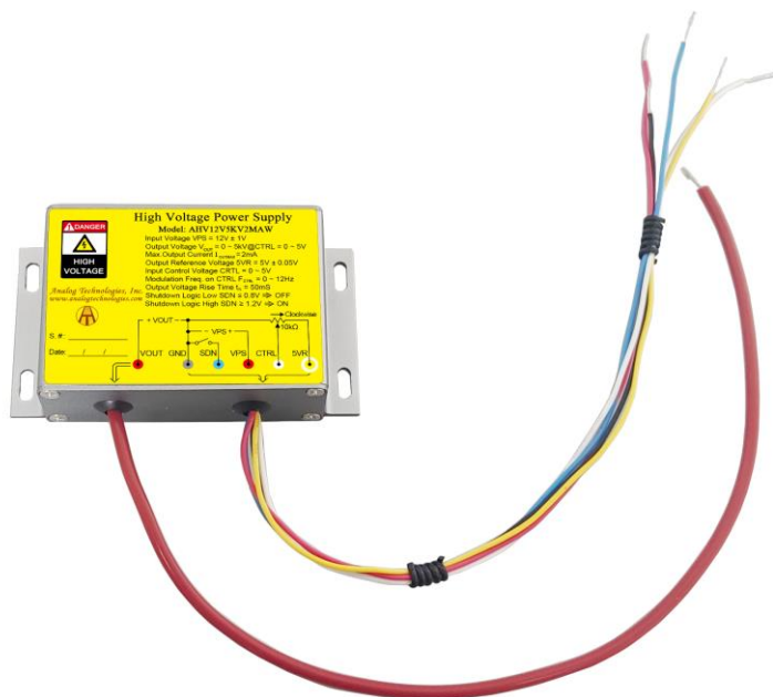
Figure 1.1. Top View of AHV12V5KV2MAW
