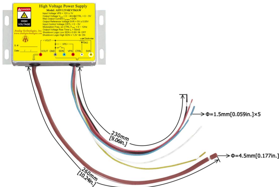
Figure 13. Connecting Lead Wires of AHV12V4KV5MAW
