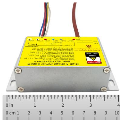
Figure 1.3. Side View
