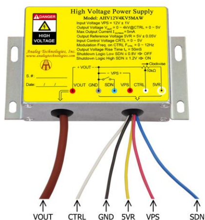
Figure 2. The Connecting Lead Wires of AHV12V4KV5MAW
