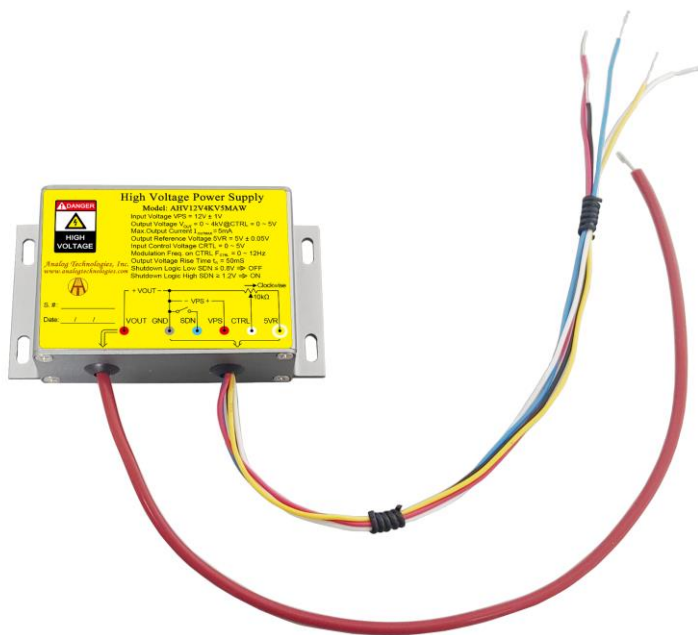
Figure 1.1. Top View of AHV12V4KV5MAW
