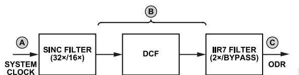
Figure 63. Decimation Filter Architecture
