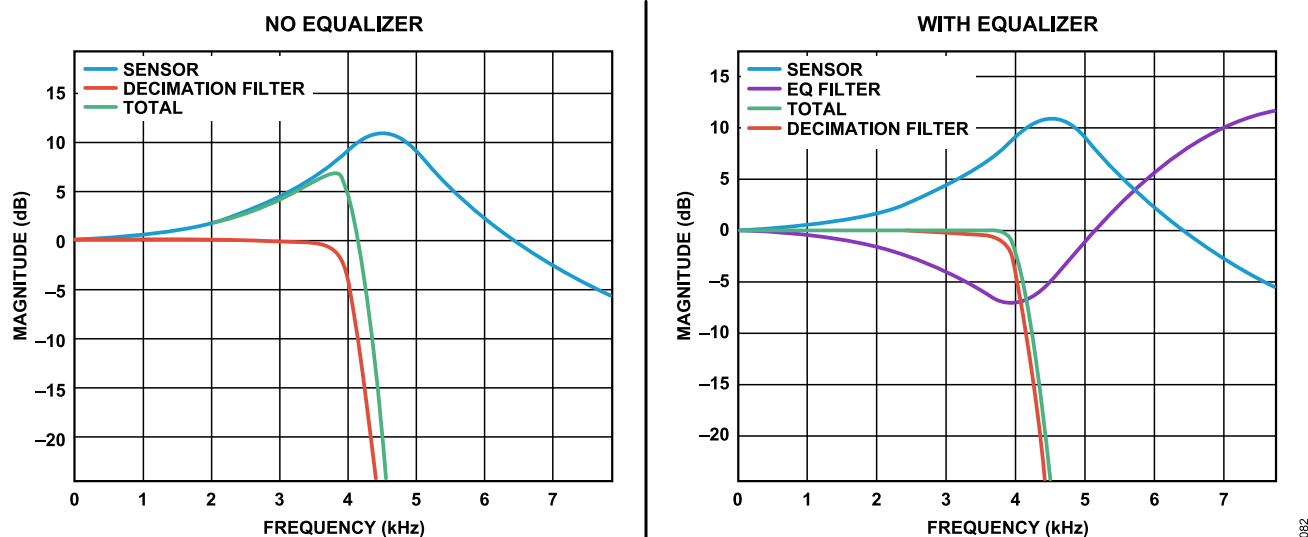
Figure 62. ADXL380 Filter Frequency Response—Equalizer Effect
