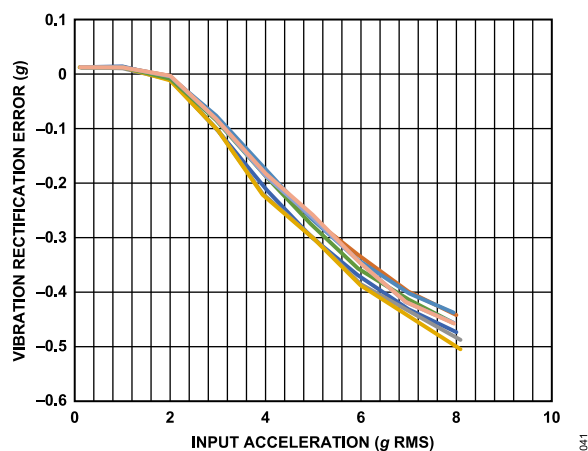
Figure 41. Y-Axis Vibration Rectification Error, Y-Axis in +1 g Field, \pm 4 g Range, V_S = 3.3 V
