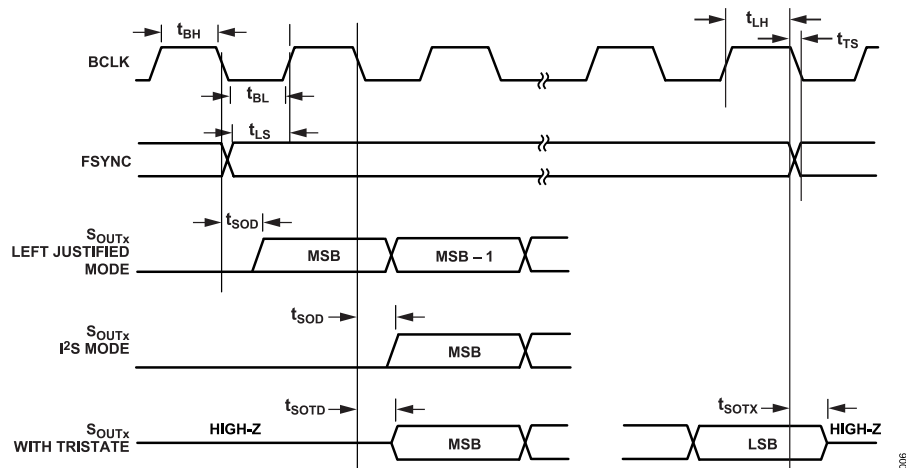
Figure 6. I²S/TDM Serial Output Port Timing Diagram
