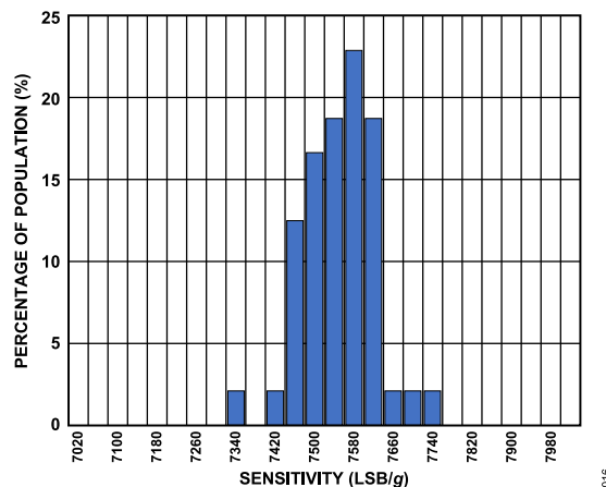
Figure 16. X-Axis Sensitivity at 25^\circ\text{C} , V_S = 3.3\text{ V} , \pm 4\text{ g} Range
