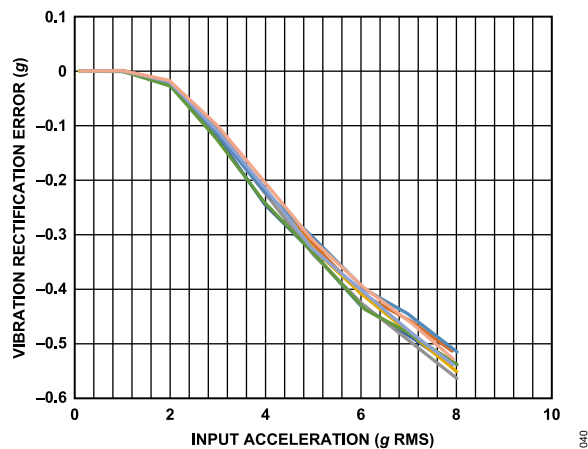
Figure 40. X-Axis Vibration Rectification Error, X-Axis in +1 g Field, \pm 4 g Range, V_S = 3.3 V
