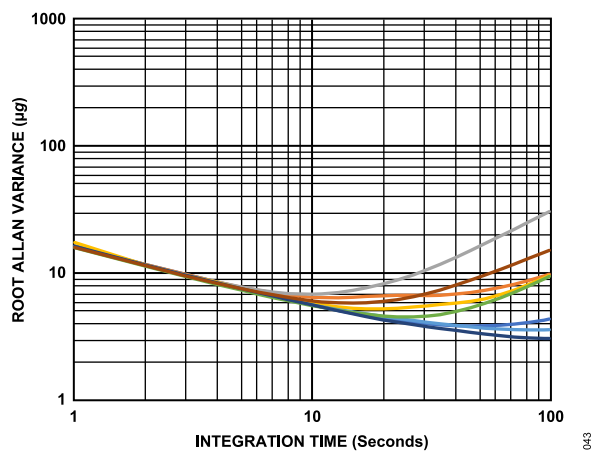
Figure 43. X-Axis Root Allan Variance at 25°C, V_S = 3.3\text{ V}
