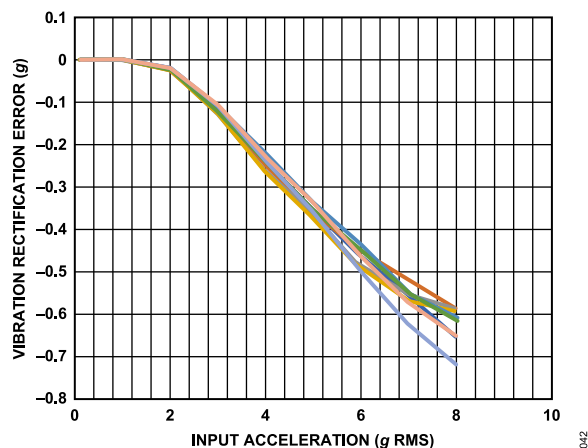
Figure 42. Z-Axis Vibration Rectification Error, Z-Axis in +1 g Field, \pm 4 g Range, V_S = 3.3 V
