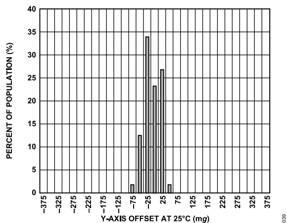
Figure 41. Zero g Offset Histogram at 25°C, Y-Axis
