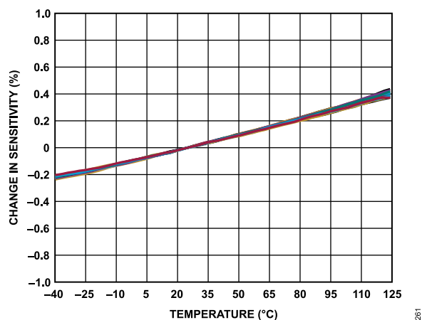
Figure 61. Sensitivity Normalized Relative to 25°C vs. Temperature X-Axis
