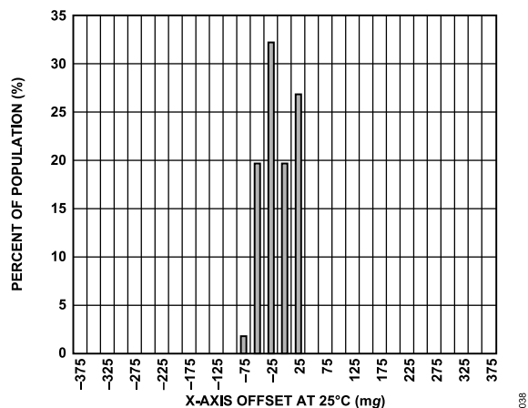
Figure 40. Zero g Offset Histogram at 25°C, X-Axis
