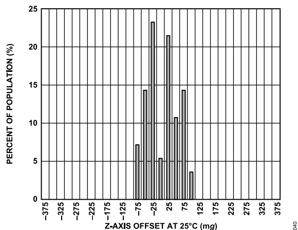
Figure 42. Zero g Offset Histogram at 25°C, Z-Axis
