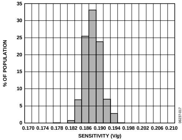
Figure 17. X-Axis Sensitivity at 25°C, V_S = 2\text{ V}
