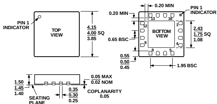
Figure 33. 16-Lead Lead Frame Chip Scale Package [LFCSP_LQ]
