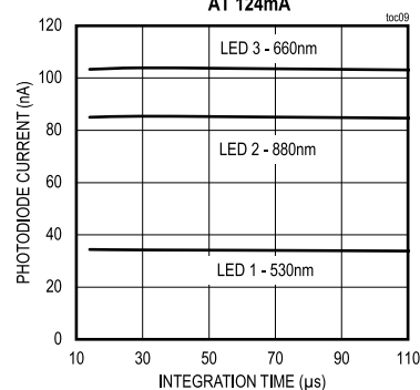
LED-PHOTODIODE CROSSTALK AT 124mA
