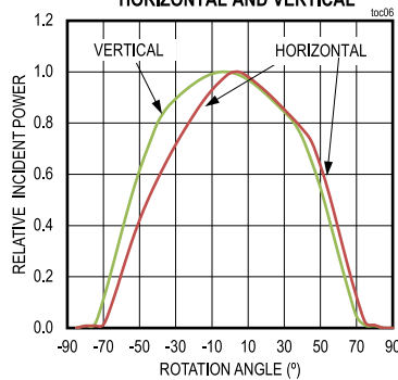
PHOTODIODE FIELD OF VIEW HORIZONTAL AND VERTICAL
