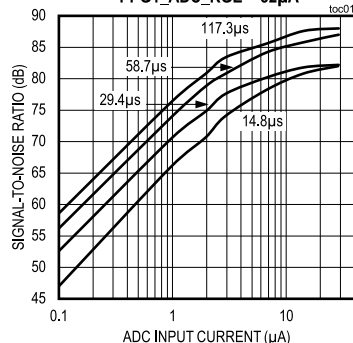
LED1 - 530nm SIGNAL-TO-NOISE RATIO vs. ADC INPUT CURRENT PPG1_ADC_RGE = 32 \mu A
