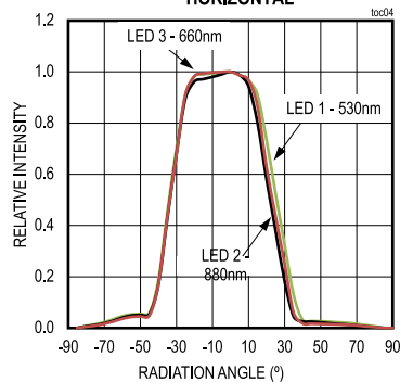
LED 2D - RADIATION PATTERN HORIZONTAL
