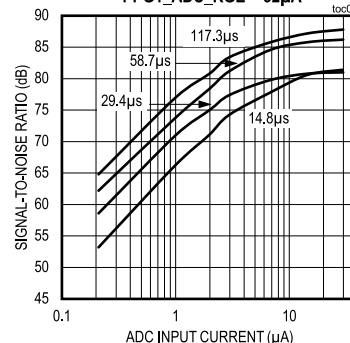
LED3 - 660nm SIGNAL-TO-NOISE RATIO vs. ADC INPUT CURRENT PPG1_ADC_RGE = 32 \mu A
