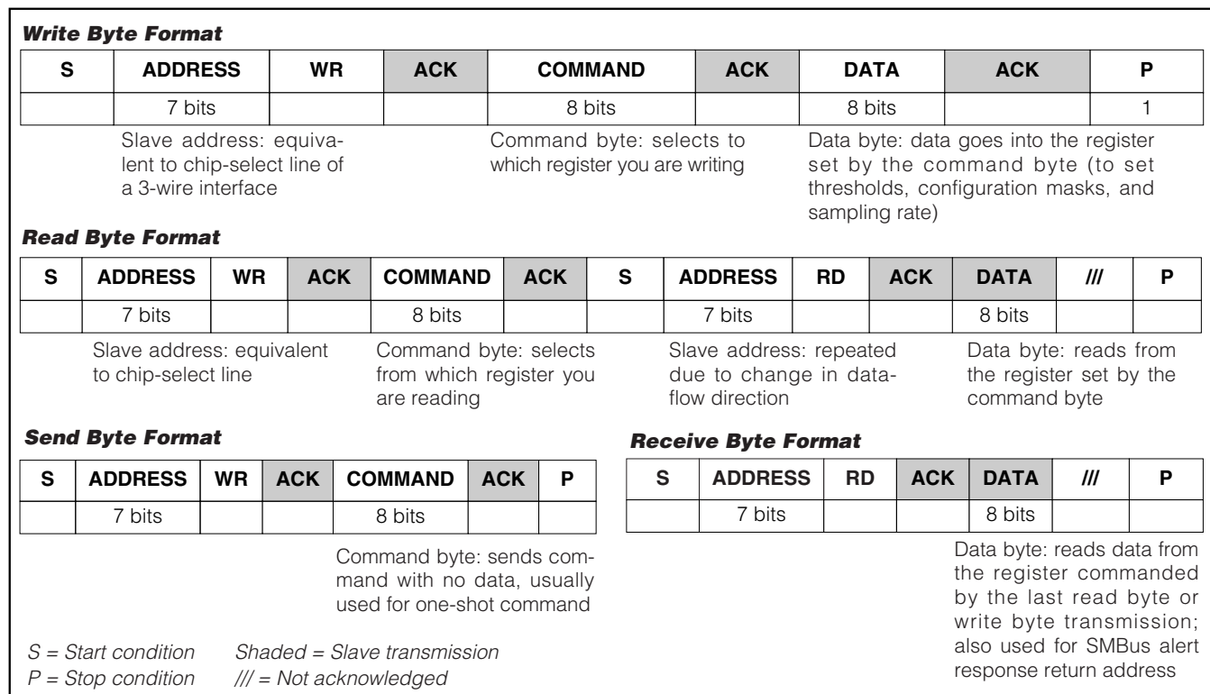
Figure 1. SMBus Protocols
