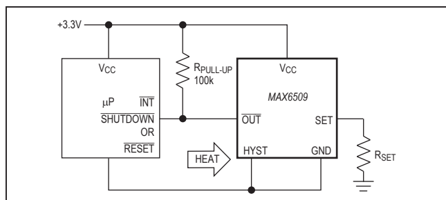
Figure 2. Microprocessor Alarm/Reset
