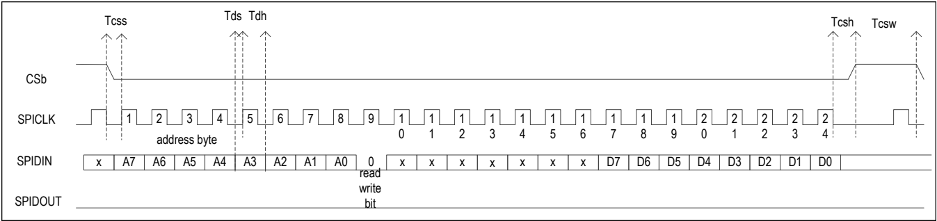
Figure 8. SPI Write
