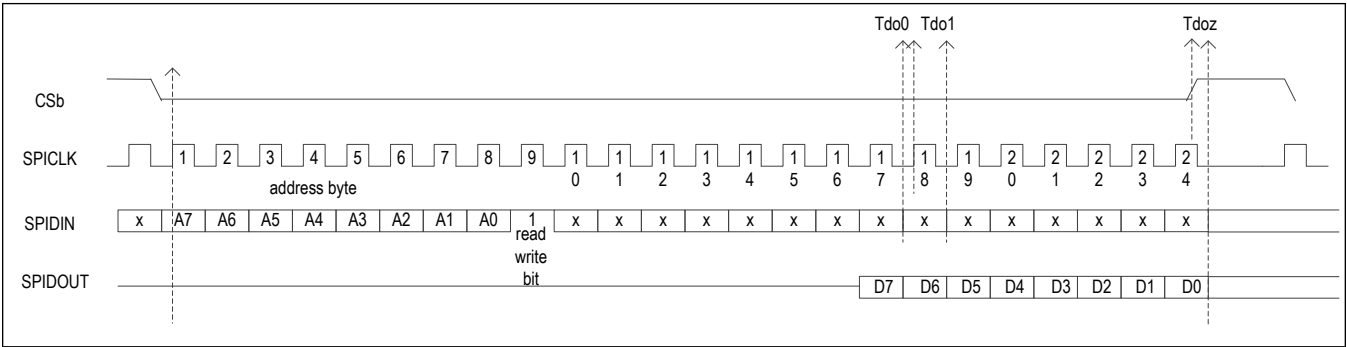
Figure 9. SPI Read
