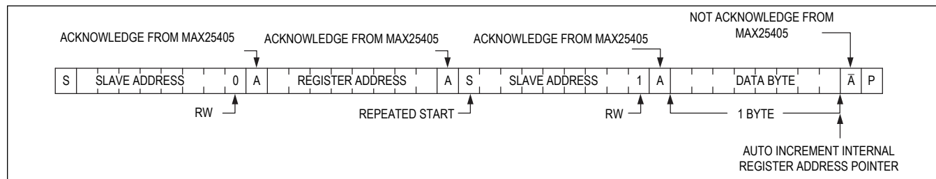
Figure 6. Reading 1 Byte of Indexed Data
