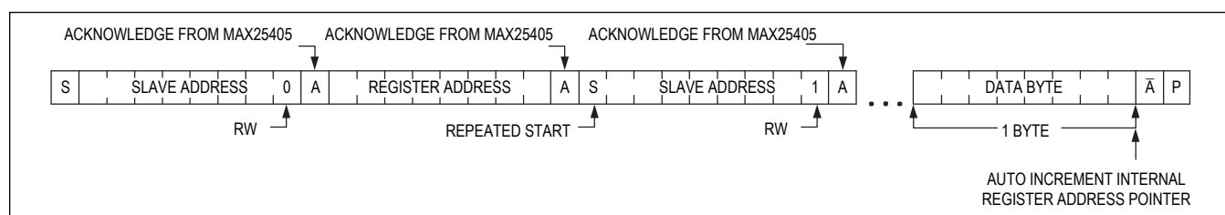
Figure 7. Reading N Bytes of Indexed Data
