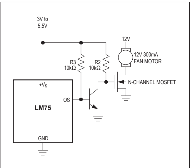
Figure 8. Fan Control
