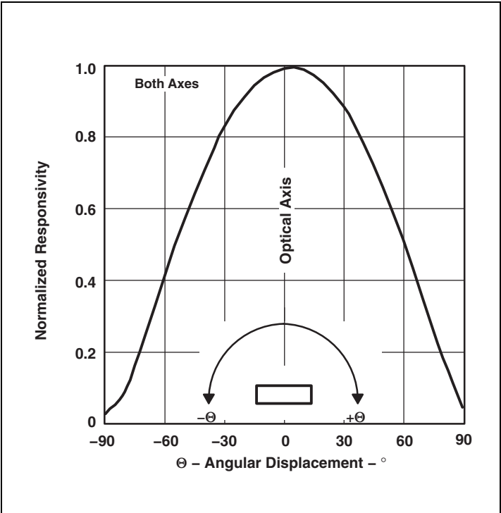
Figure 15: Normalized Responsivity vs. Angular Displacement
