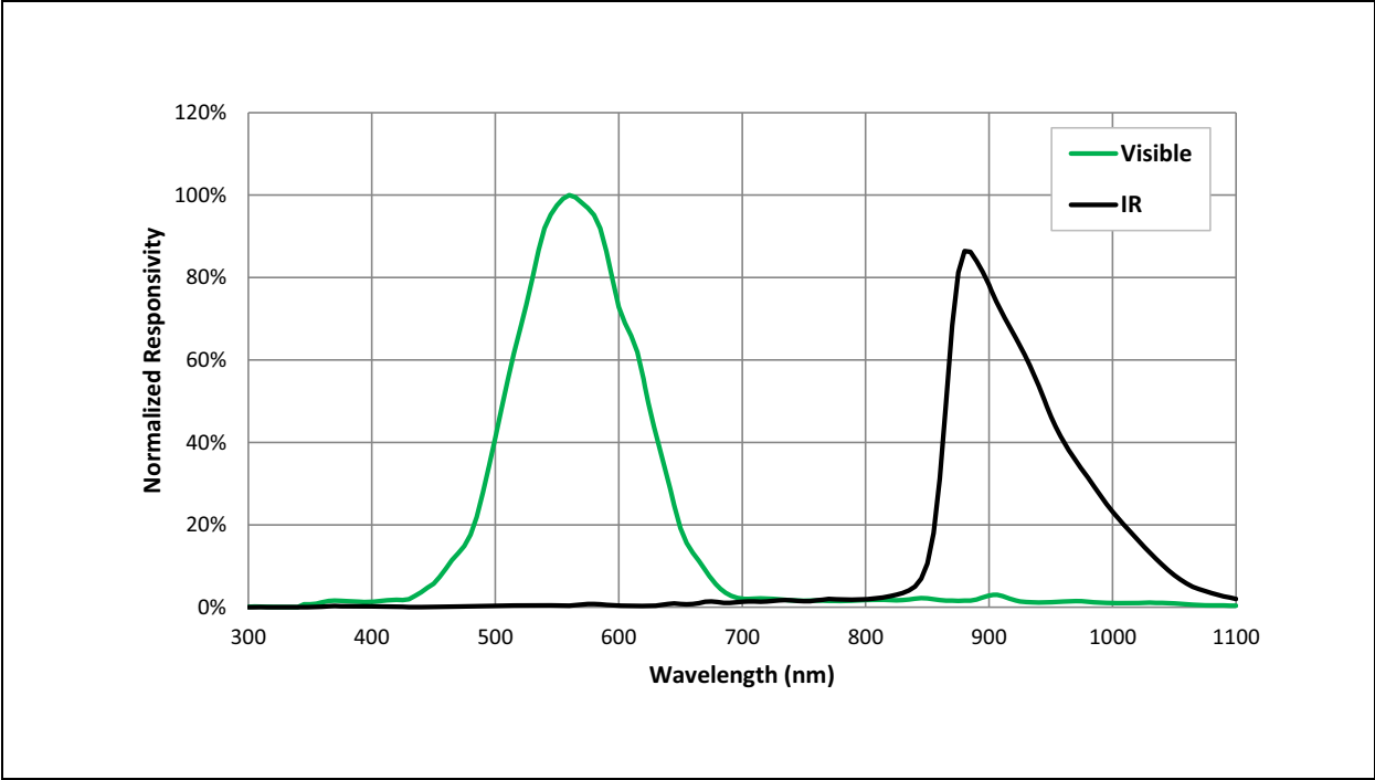
Figure 9: Spectral Responsivity
