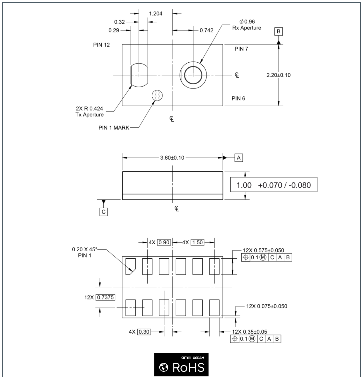
Figure 125: Package Drawing
