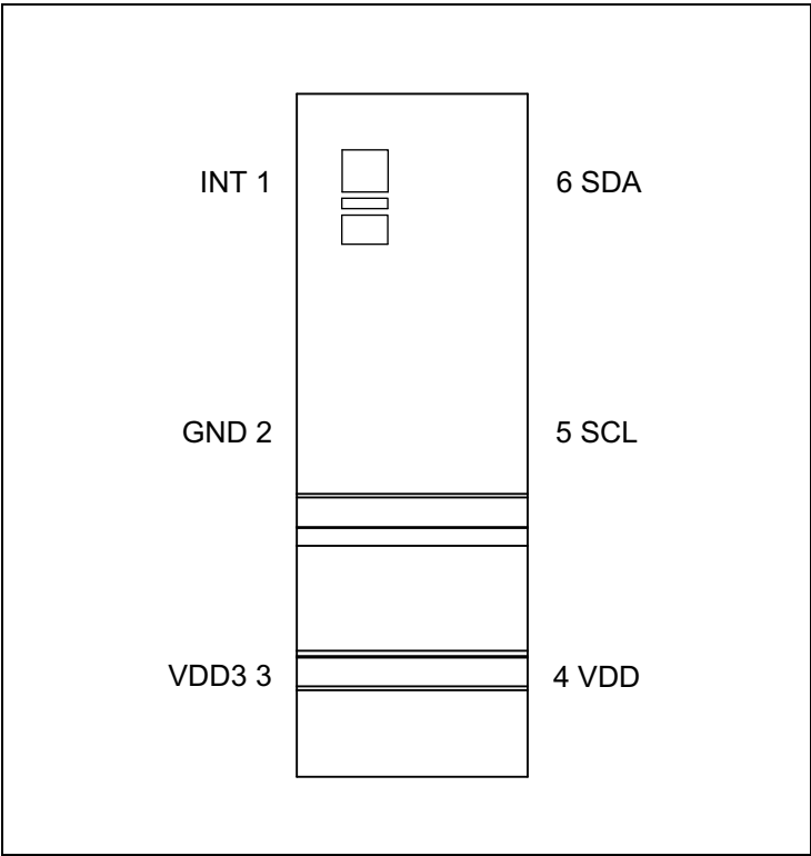
Figure 3: Pin Diagram
