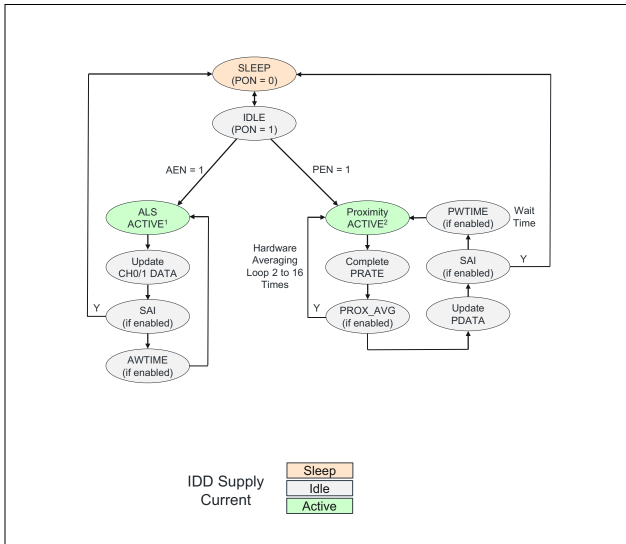
Figure 14: Operational State Diagram
