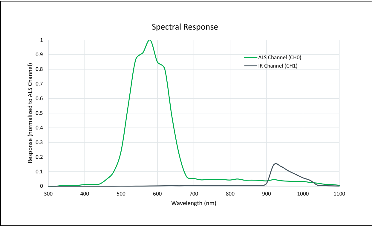
Figure 12: Spectral Responsivity
