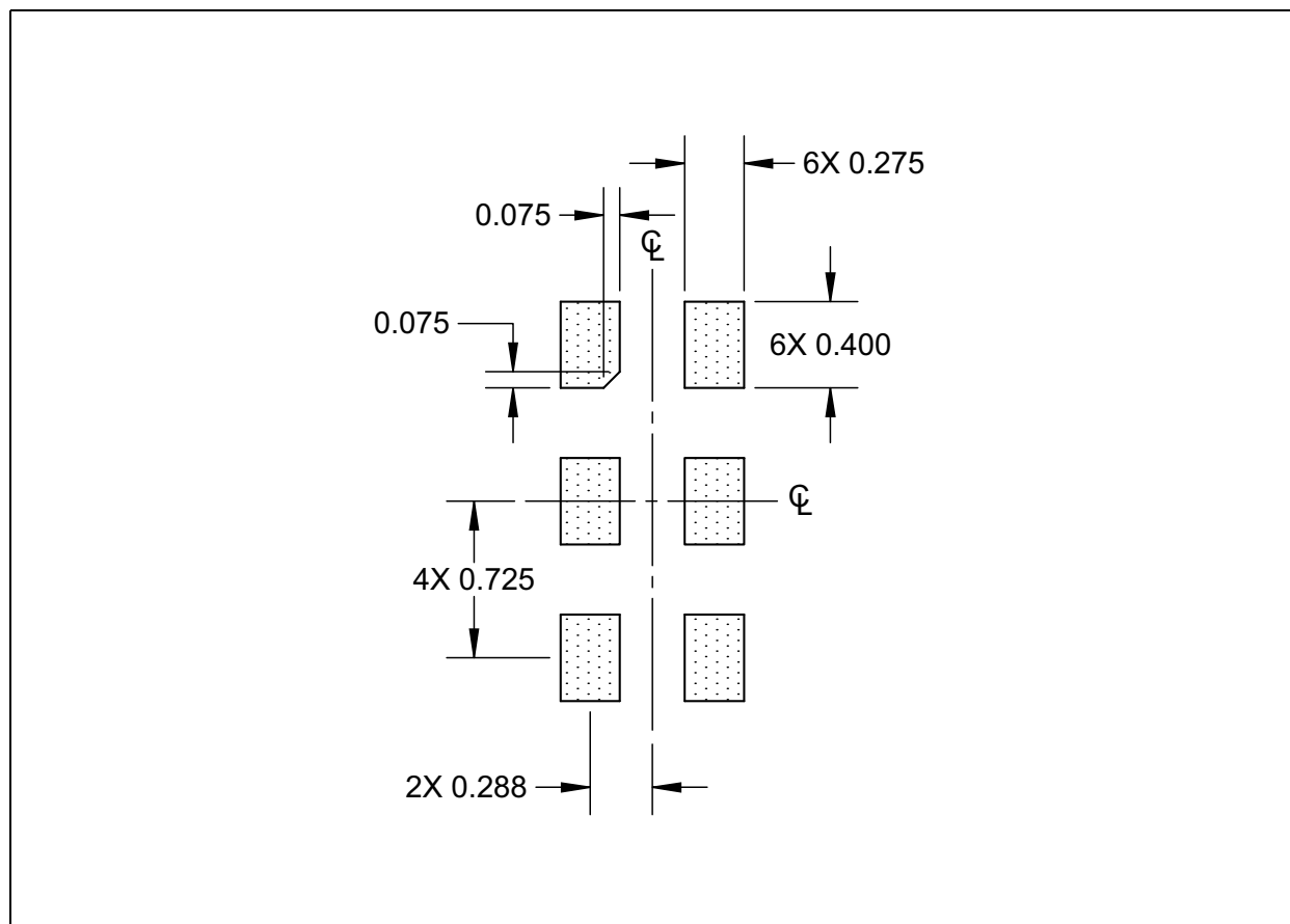
Figure 63: Recommended PCB Pad Layout
