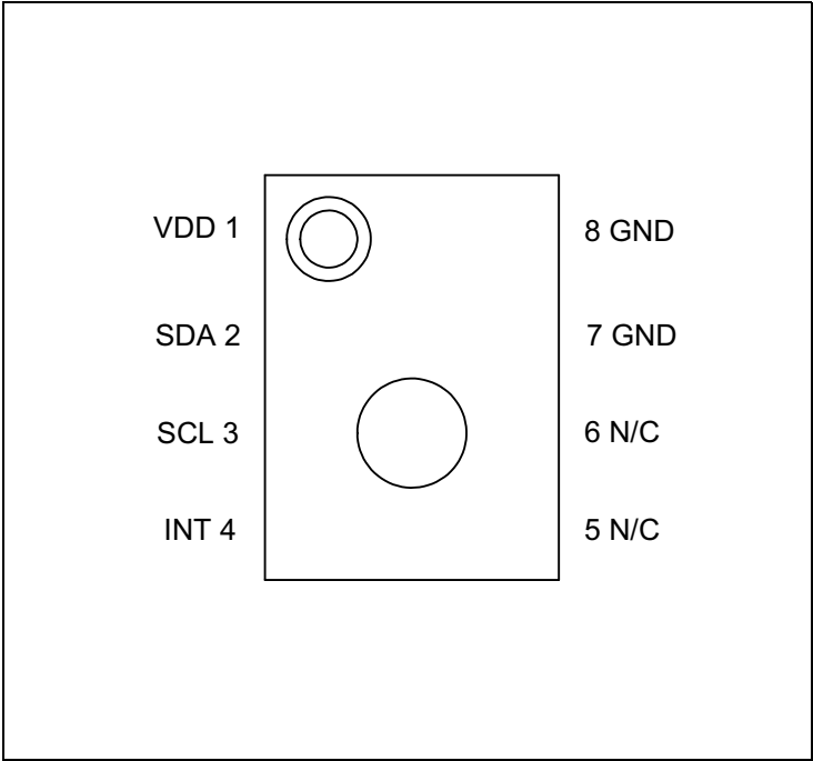
Figure 3: TCS3430 Pinout (Top View)
