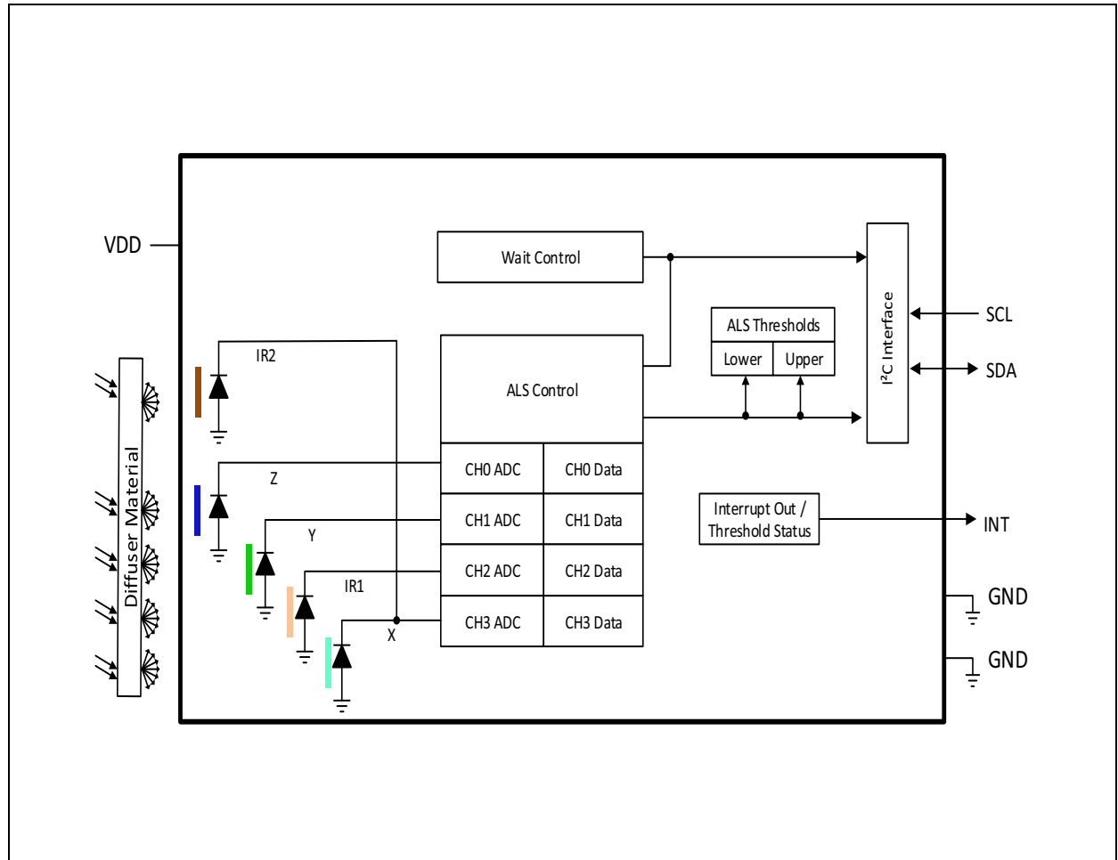
Figure 2: TCS3430 Block Diagram
