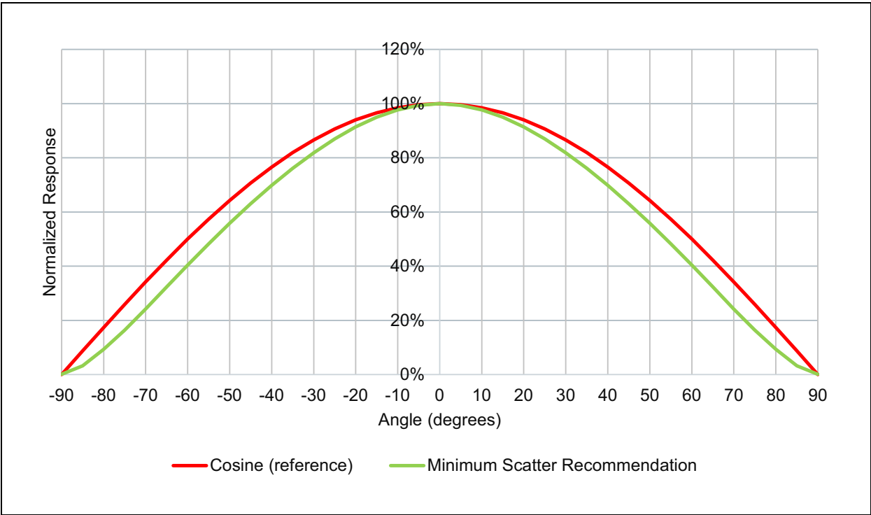
Figure 40: Diffuser Characteristics
