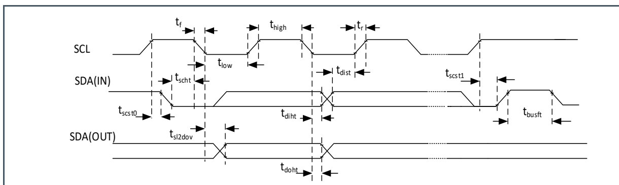
Figure 25: I 2 C Interface Timing
