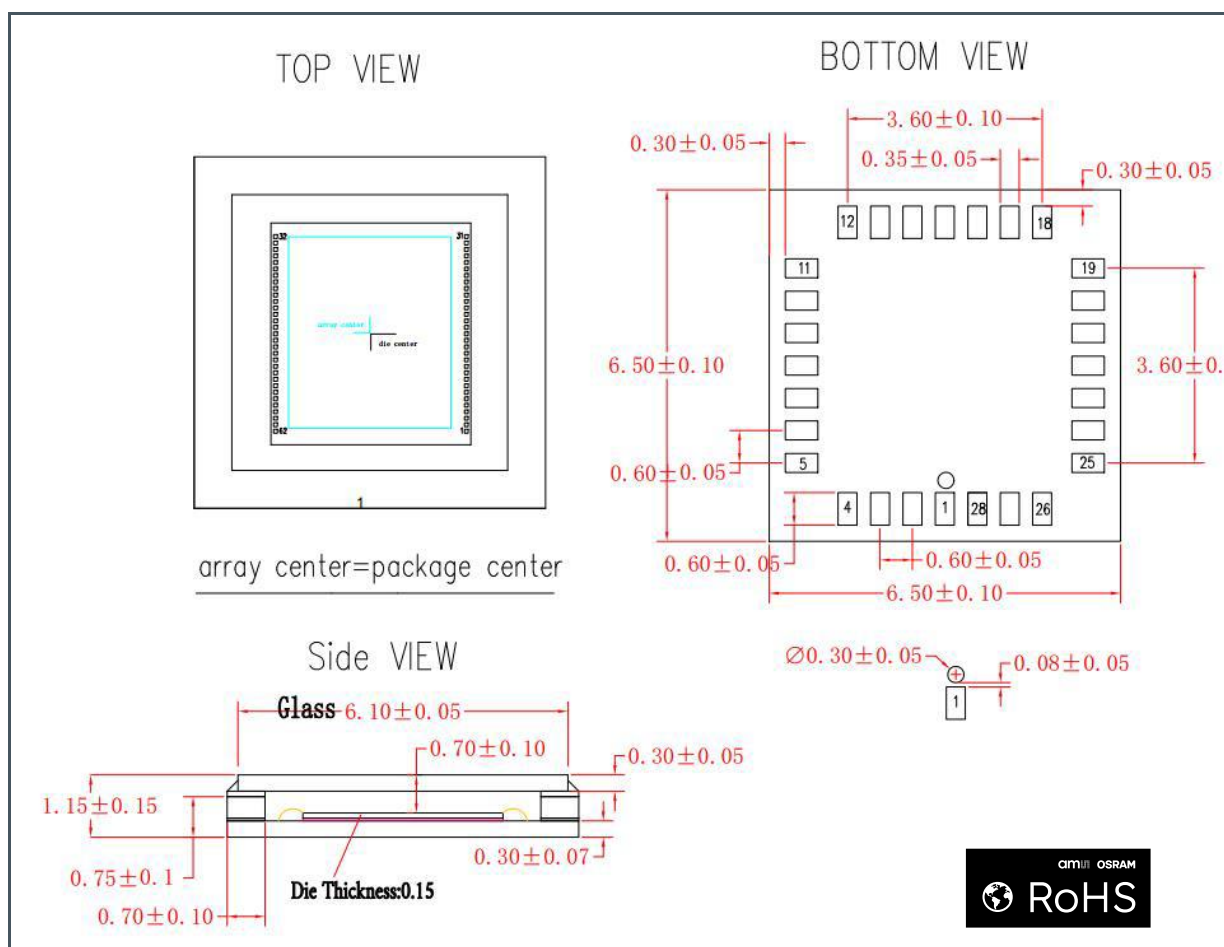
Figure 5: Mira130-1QM2PP PLCC Package Dimension
