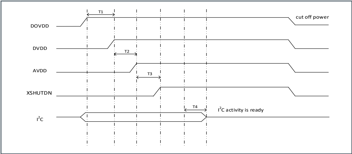
Figure 19: Power-Up Sequence
