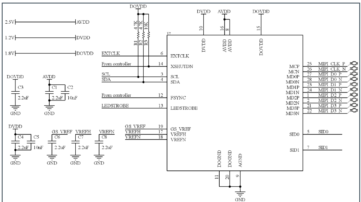
Figure 11: Application Circuit for PLCC Package
