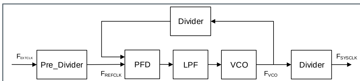
Figure 35: PLL Block Diagram
