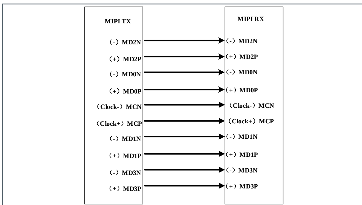
Figure 28: MIPI Interface
