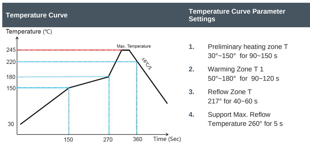
Figure 6: Temperature Curve and Timing Settings
