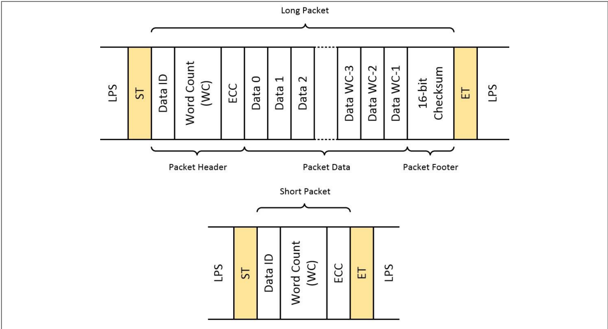
Figure 12: MIPI long & short packet structure
