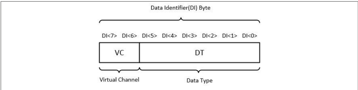
Figure 14: MIPI data packet DI structure
