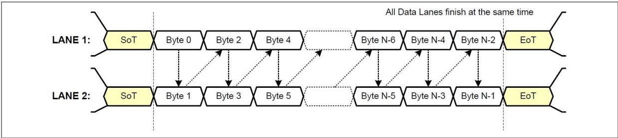
Figure 13: MIPI 2-lane data package transmission
