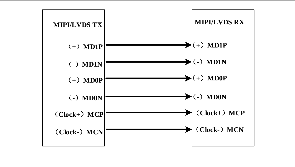
Figure 10: MIPI/LVDS interface
