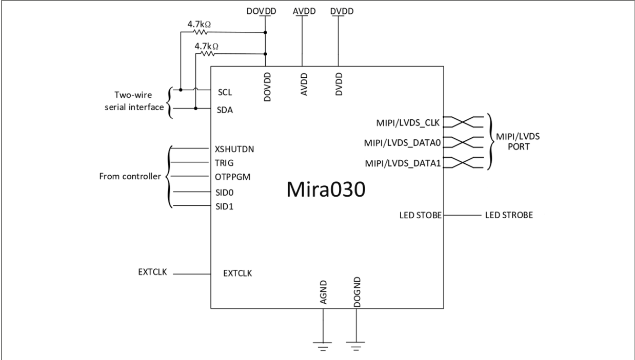
Figure 2: Typical configuration
