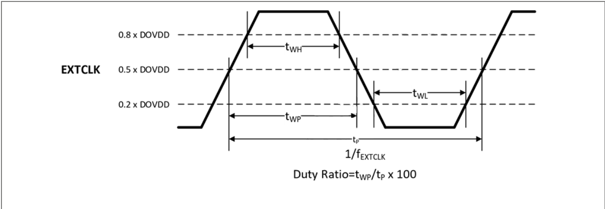
Figure 5: Input clock waveform
