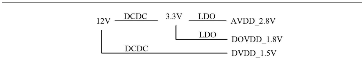
Figure 26: Power tree recommendation
