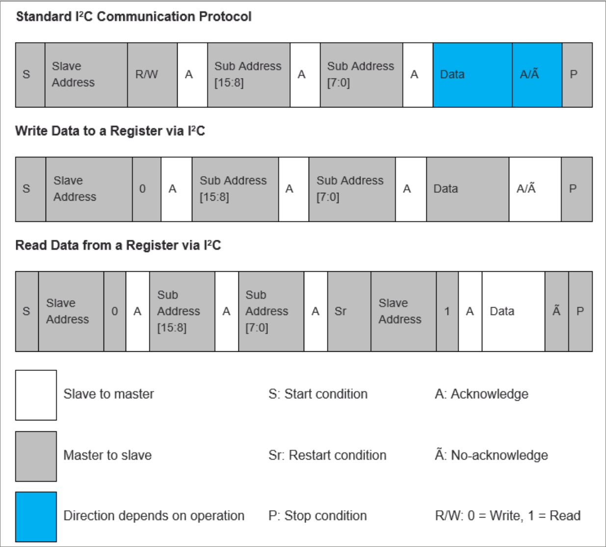
Figure 8: I²C bus device address control example
