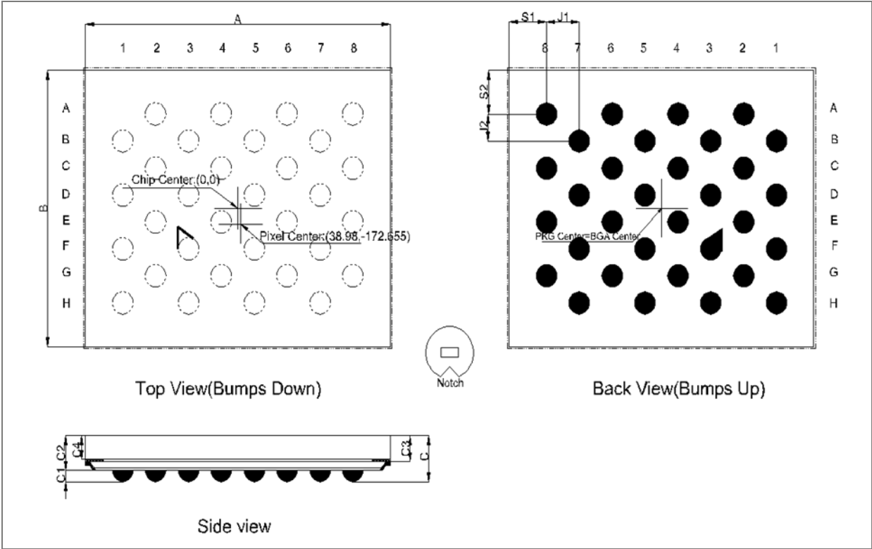
Figure 28: Package drawing
