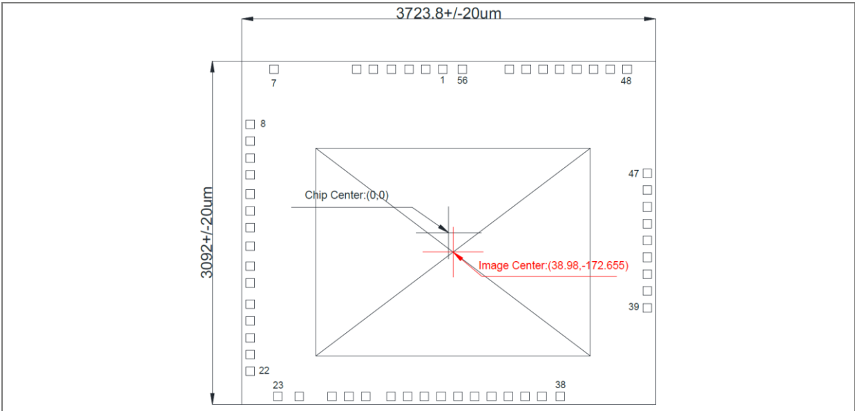
Figure 3: Mira030 RW package pin assignment
