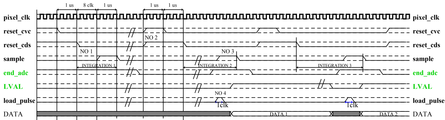
Fig 20: Timing diagram
