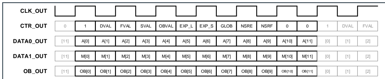
Figure 54: Low-Level Pixel Timing (per side)
