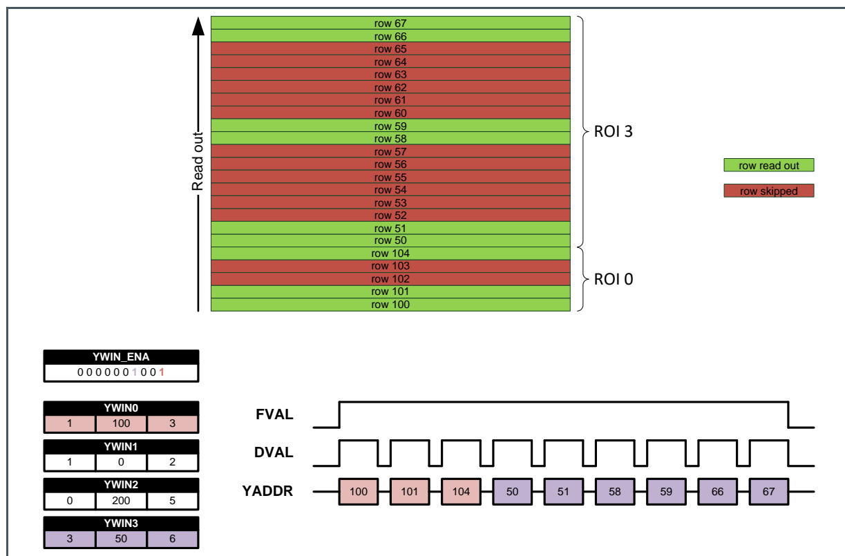
Figure 102: Vertical ROI Example (color mode)
