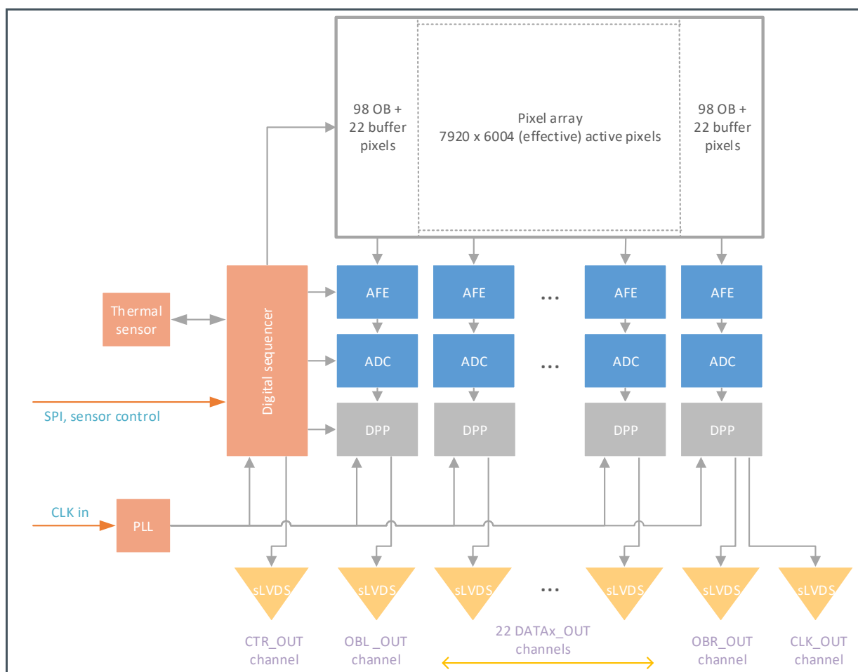
Figure 2: Functional Blocks of CMV50000
