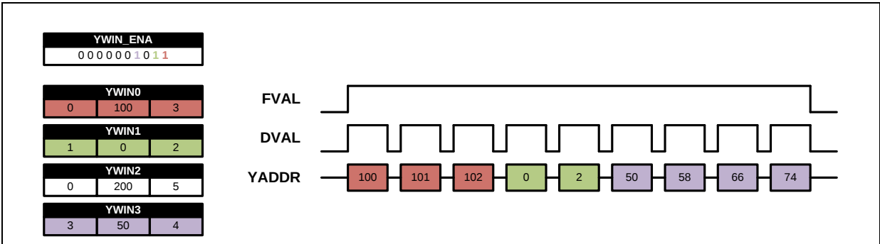
Figure 98: Vertical ROI Example (monochrome)
