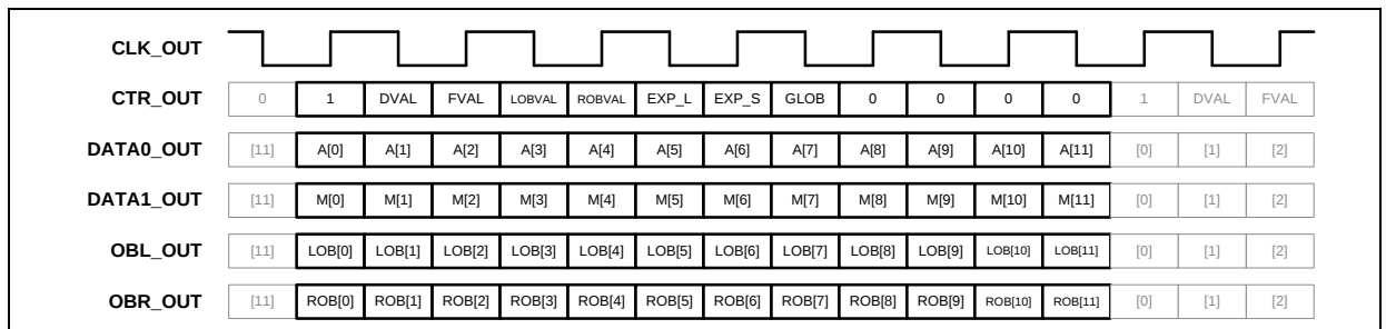
Figure 54: Low-Level Pixel Timing
