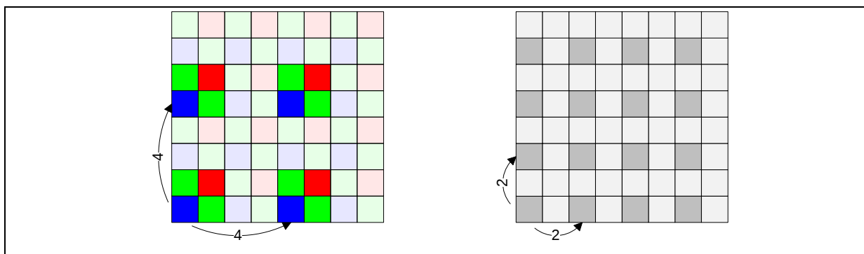
Figure 103: XY-Subsampling for Color and Mono Sensors
