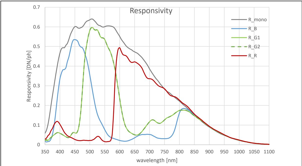
Figure 9: Responsivity (Analog Gain x4)
