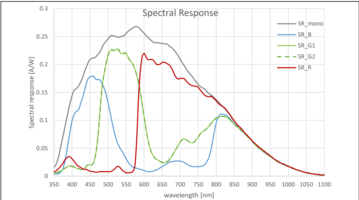
Figure 10: Spectral Response
