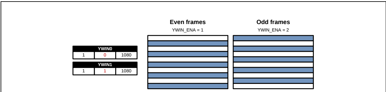
Figure 99: Interleaved Readout
