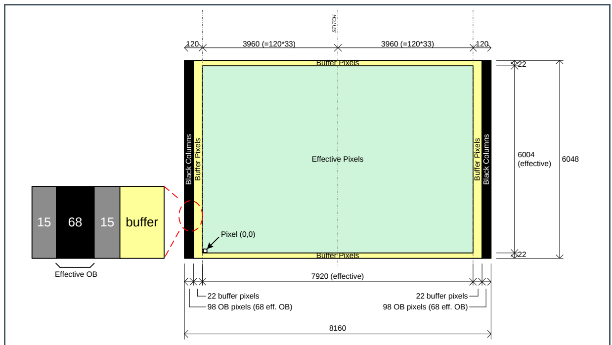
Figure 14: Pixel Array
