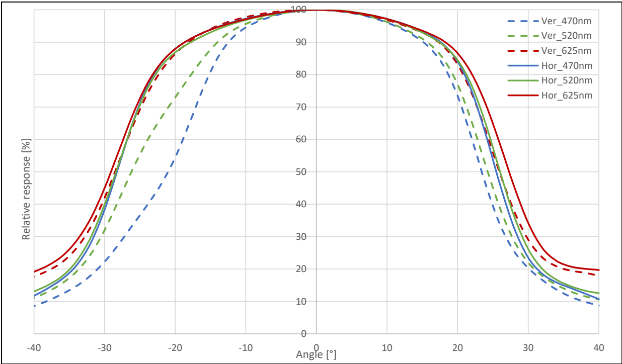
Figure 13: Angular Response
