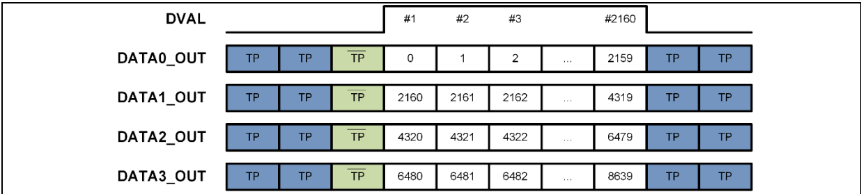
Figure 112: Multiplexed Sub-LVDS Timing Example
