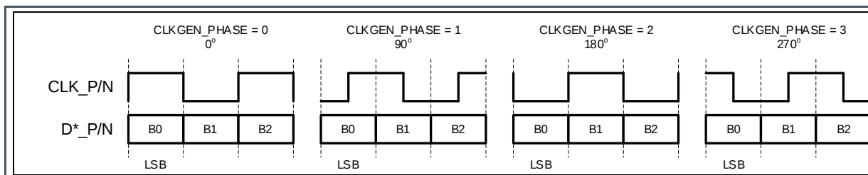
Figure 58: Output Clock: Phase Programmability
