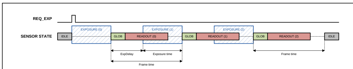
Figure 46: Timing Diagram: Triggered Internal Mode
