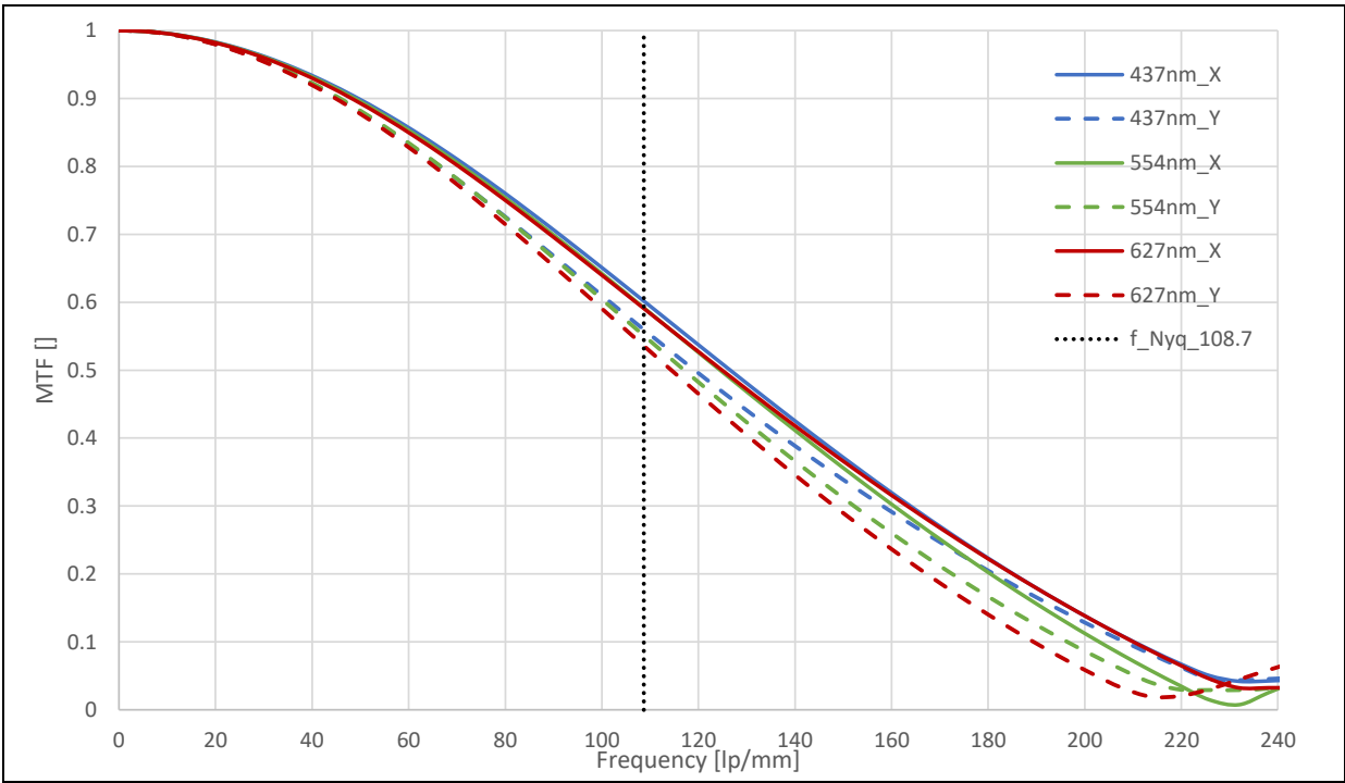
Figure 12: MTF
