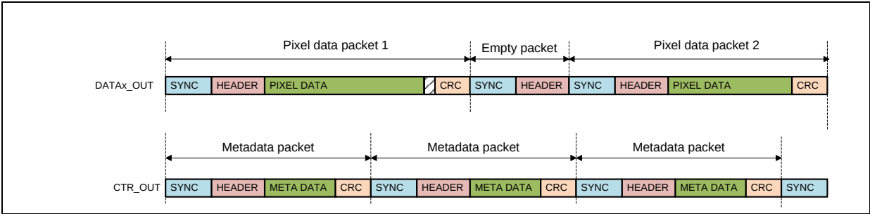
Figure 60: Low-Level Packet Timing
