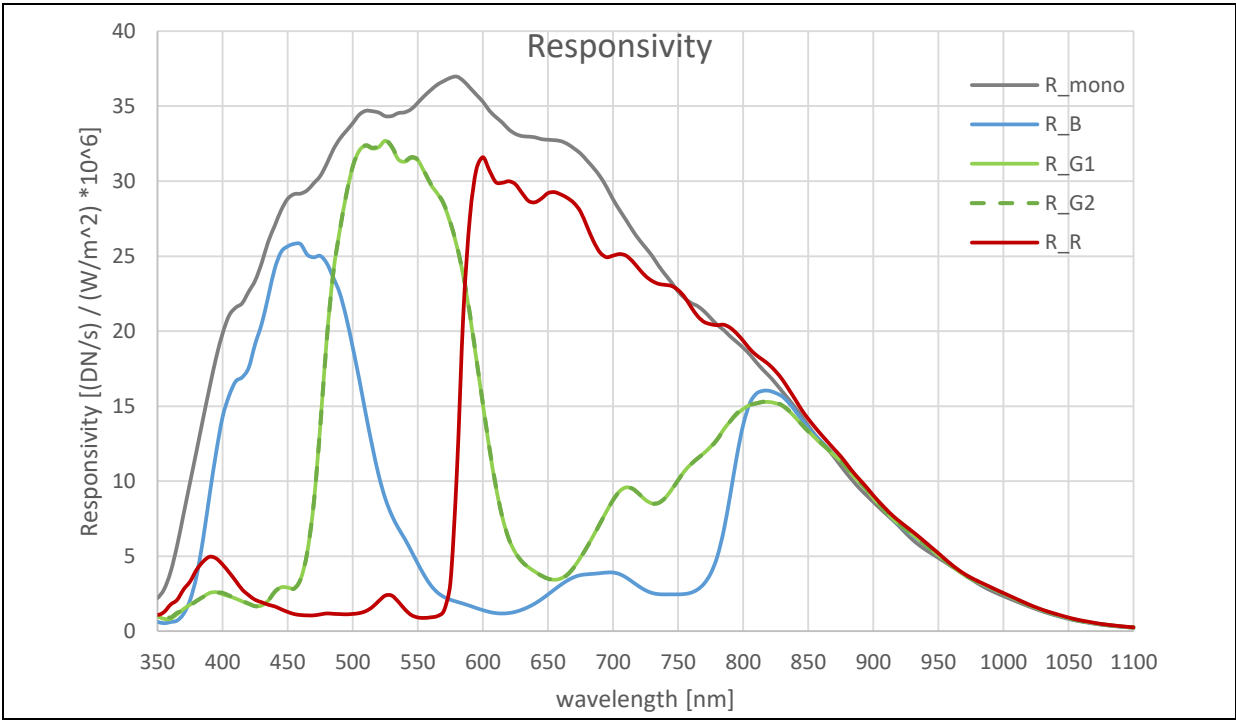
Figure 11: Responsivity (Analog Gain x4)
