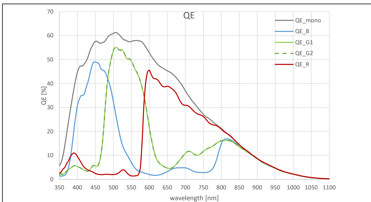
Figure 8: Quantum Efficiency
