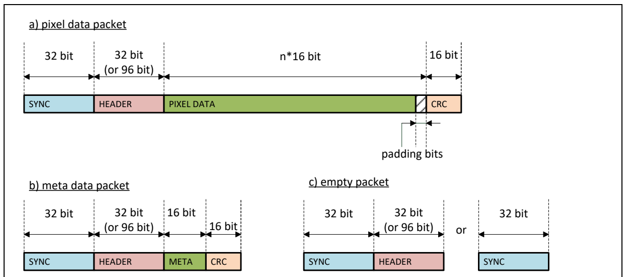
Figure 59: Packet Types
