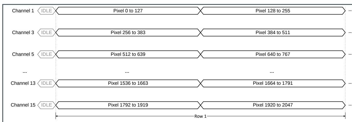
Figure 43: Pixel Remapping for 8 Output Channels
