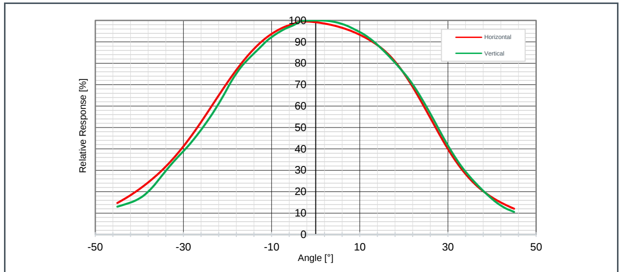
Figure 12: Horizontal and Vertical Angular Response
