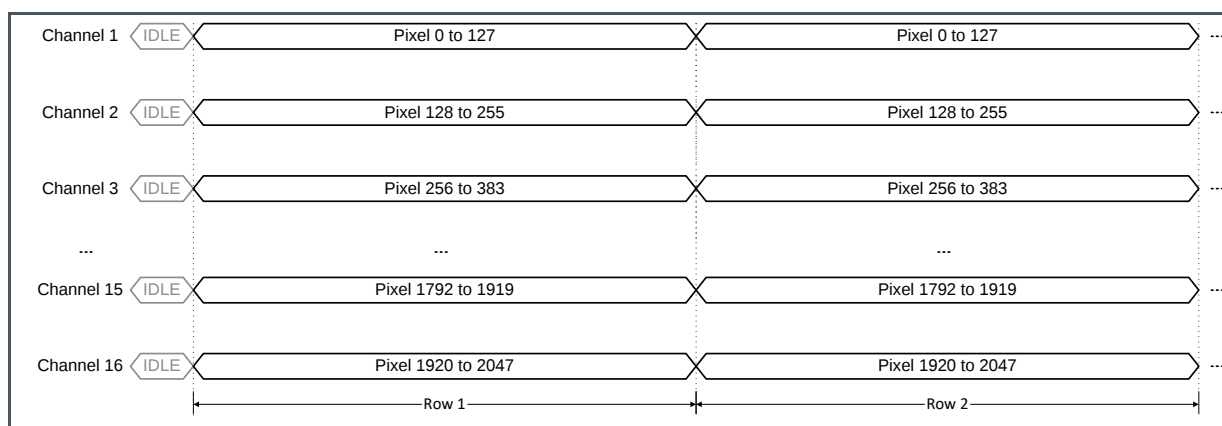
Figure 42: Pixel Remapping for 16 Output Channels
