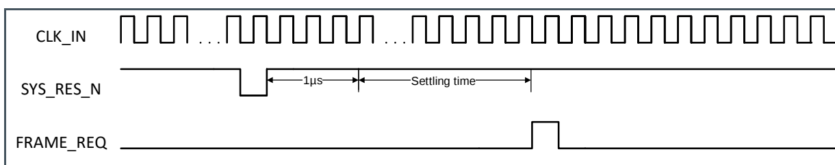
Figure 23: Reset Sequence
