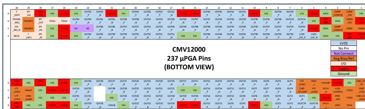
Figure 100: Pin Layout from Bottom View
