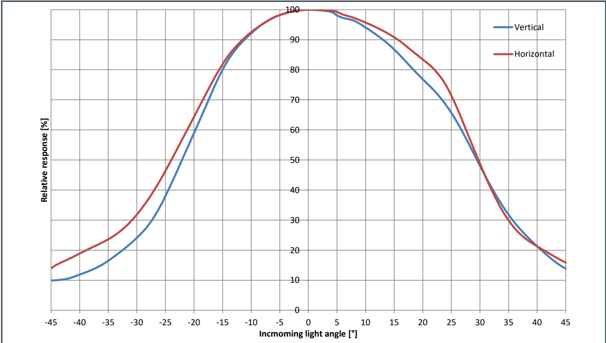
Figure 10: Angular Response
