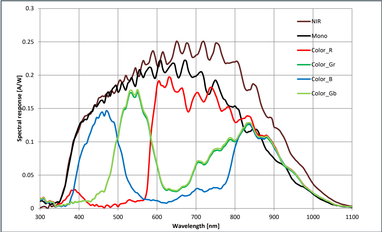
Figure 9: Spectral Response
