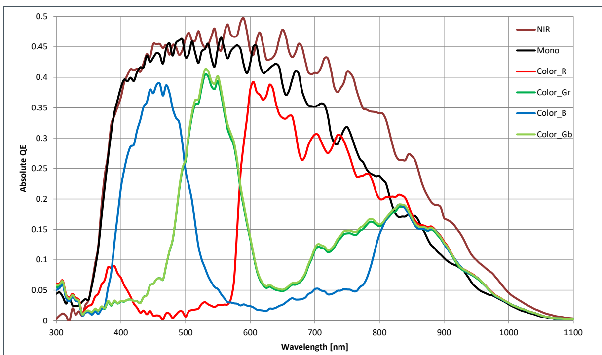
Figure 8: Quantum Efficiency
