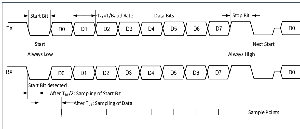
Figure 26: UART Protocol
