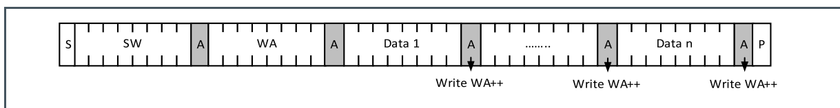
Figure 21: I 2 C Page Write
