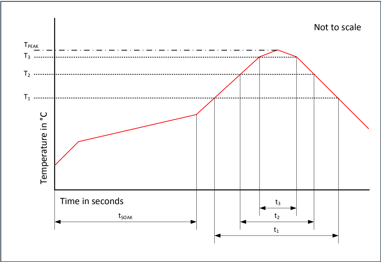
Figure 41: Solder Reflow Profile Graph
