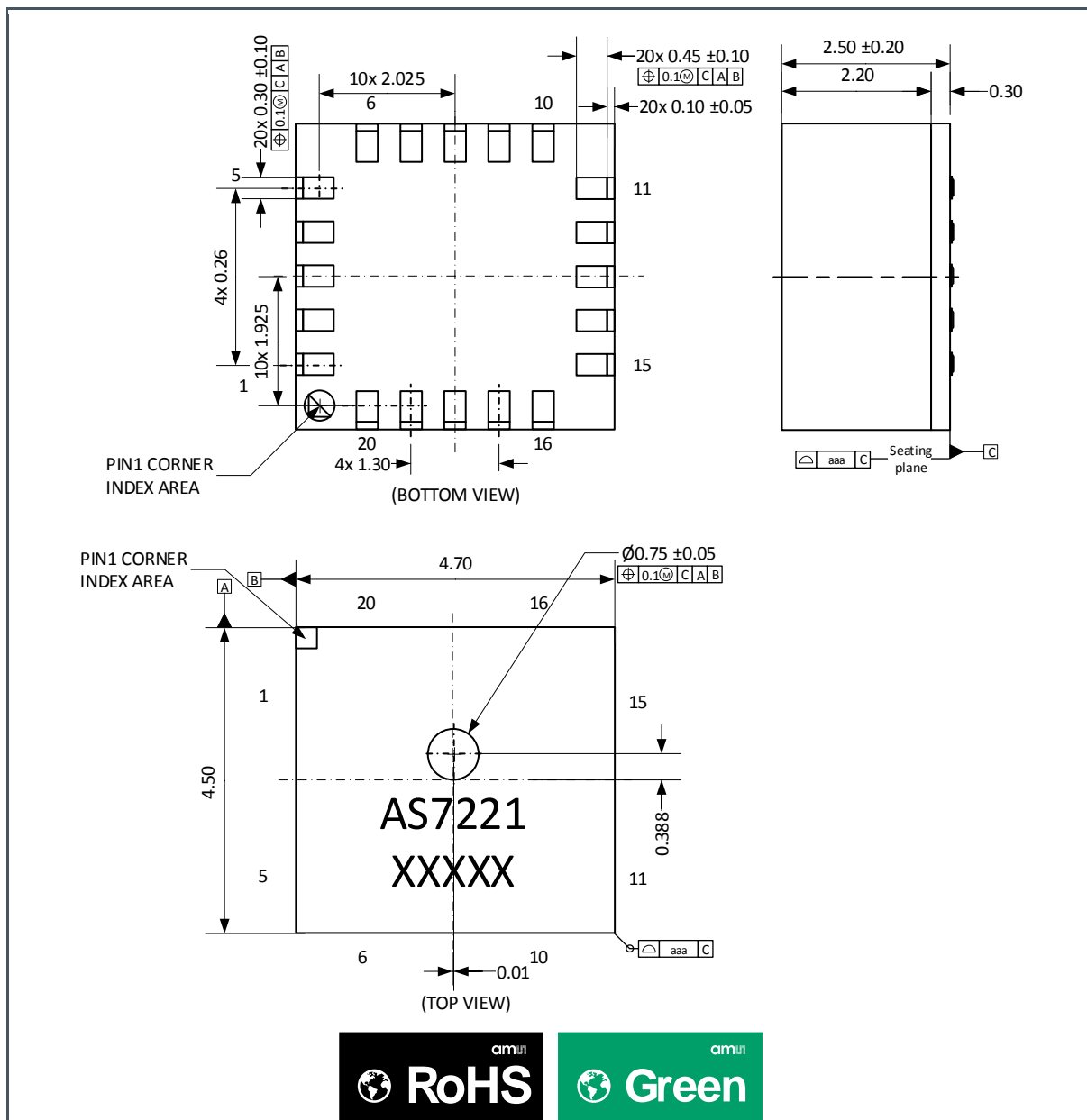
Figure 38: 20-Pin LGA Package Outline Drawing (Front Side Marking)
