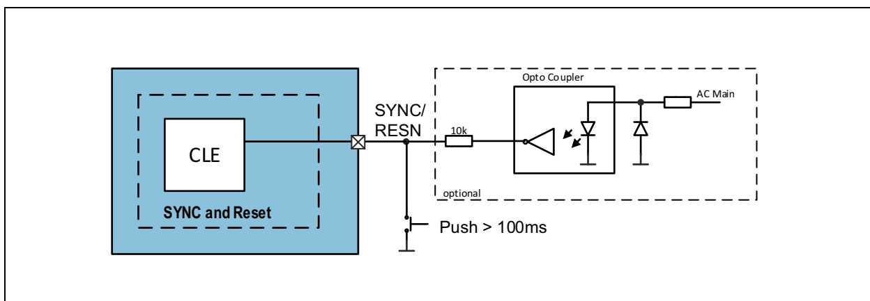
Figure 19: Synchronization and Reset Circuit
