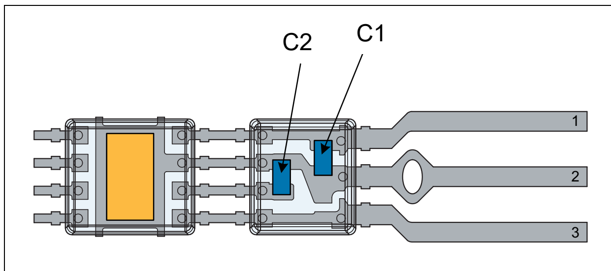
Figure 73: AS5172E/F Components
