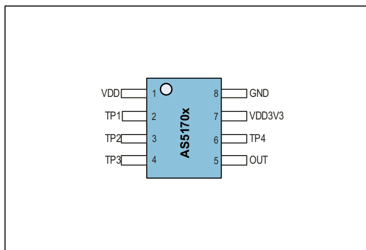
Figure 5: AS5170A/B/C/D Pin Assignment (Top View, SOIC8)
