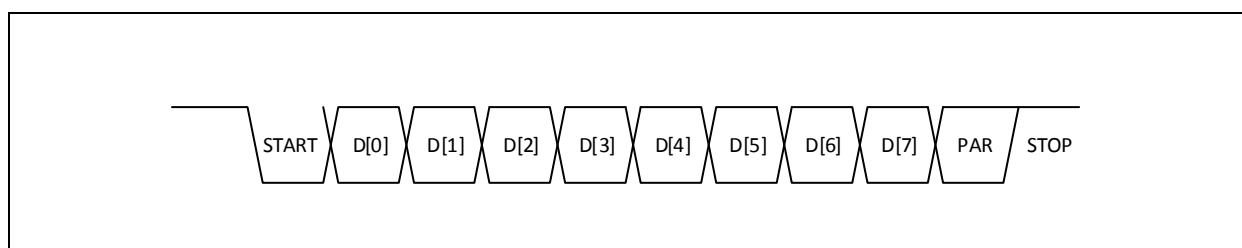
Figure 19: UART Frame
