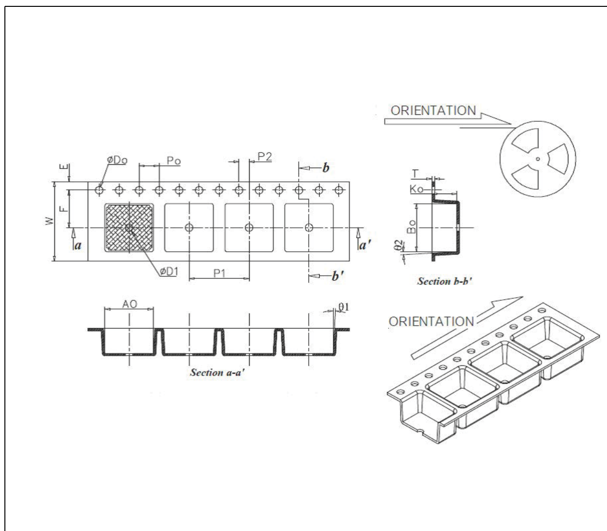
Figure 18: Tape and Reel Information
