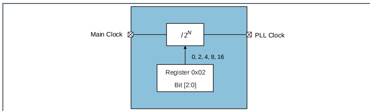
Figure 43: Internal Clock Generation
