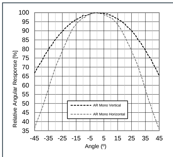
Figure 23: 4LS Monochrome Relative Angular Response (1)
