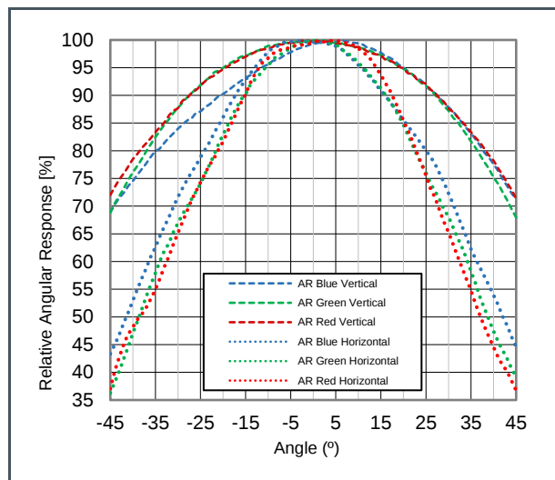
Figure 24: 4LS RGB Relative Angular Response (1)(2)
