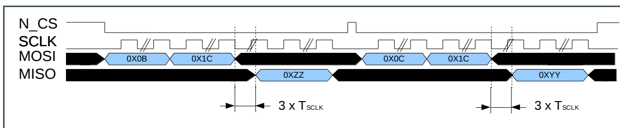
Figure 85: Read Cycle For Multiple Registers
