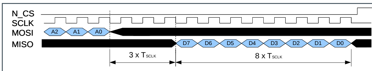
Figure 84: Read Back Data in Detail
