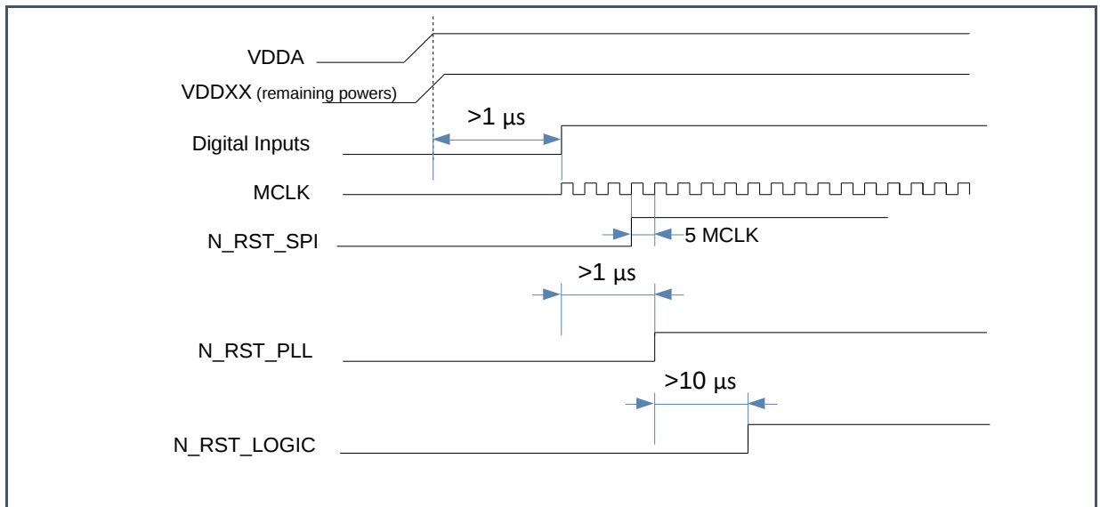
Figure 33: Power-On Sequence
