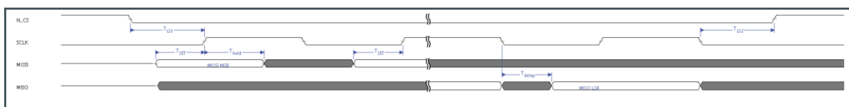
Figure 89: Time Guard Between Signals
