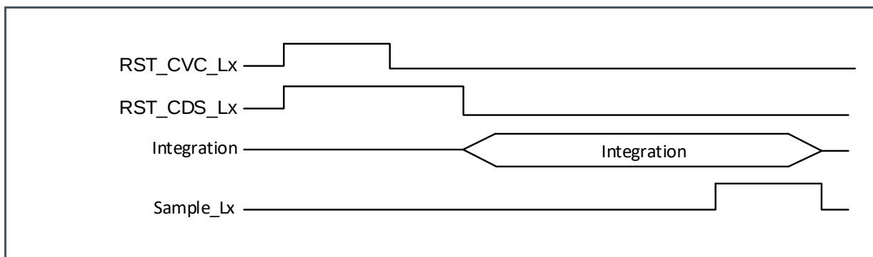
Figure 31: Standard Mode Operation
