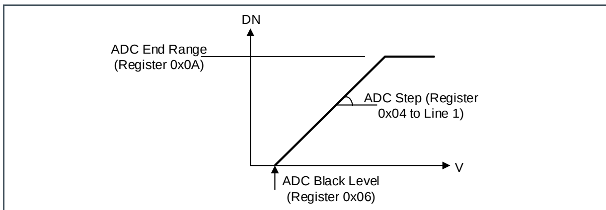
Figure 34: ADC Transfer Function in Linear Mode
