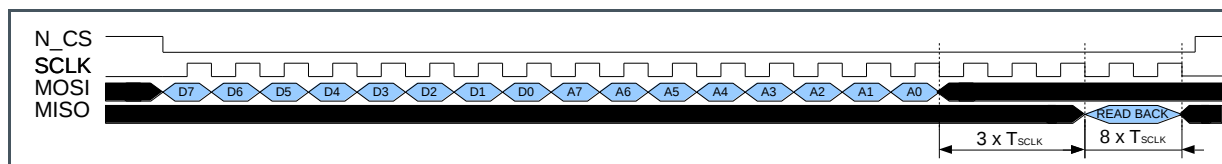
Figure 83: Read Cycle Over SPI Interface
