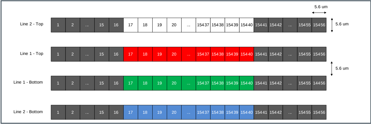
Figure 28: Pixel Distribution on 4LS15K RGB + Monochrome
