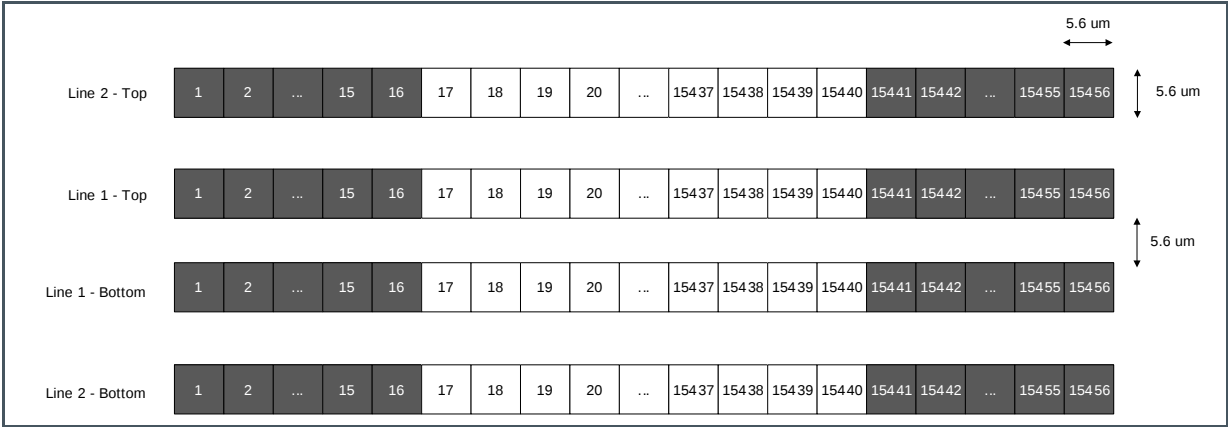
Figure 29: Pixel Distribution on 4LS15K Monochrome
