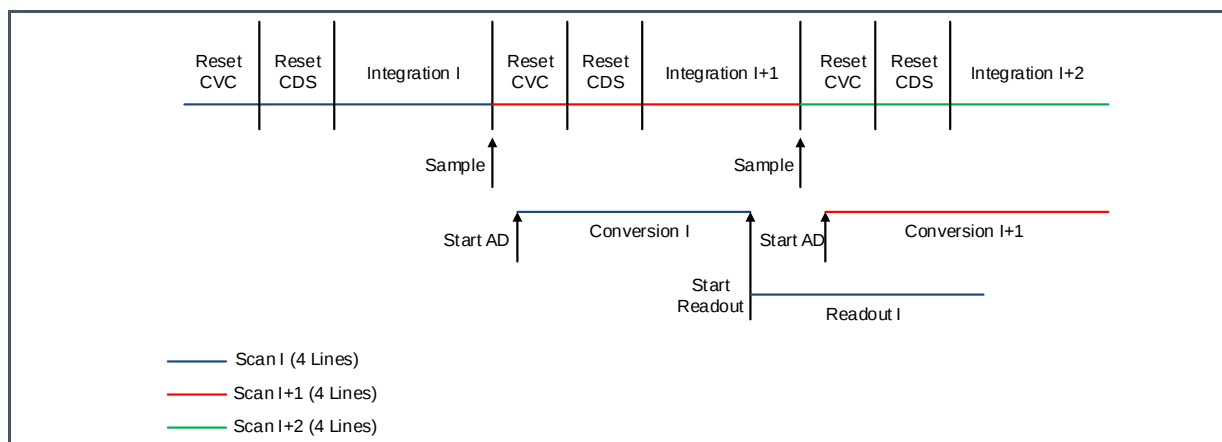
Figure 32: 4LS Pipeline Overview
