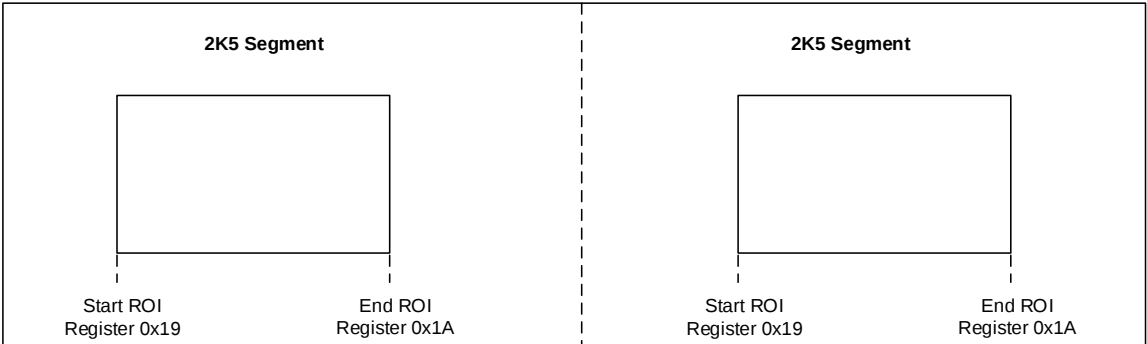
Figure 70: Centered ROI
