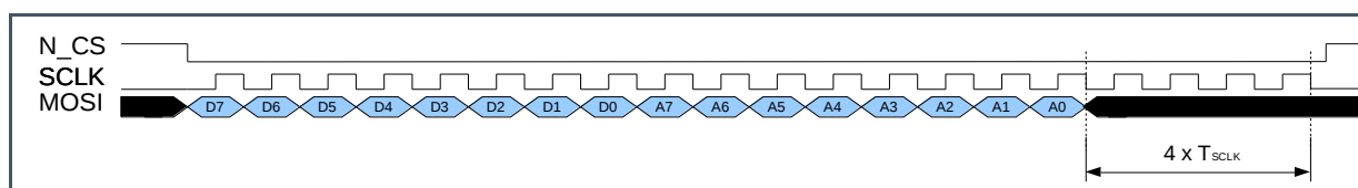
Figure 81: Write Cycle Over SPI Interface
