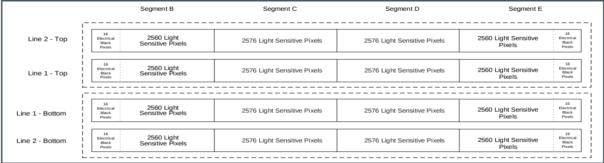
Figure 26: 4LS10K Sensor with Four Stitched 2K5 Segments
